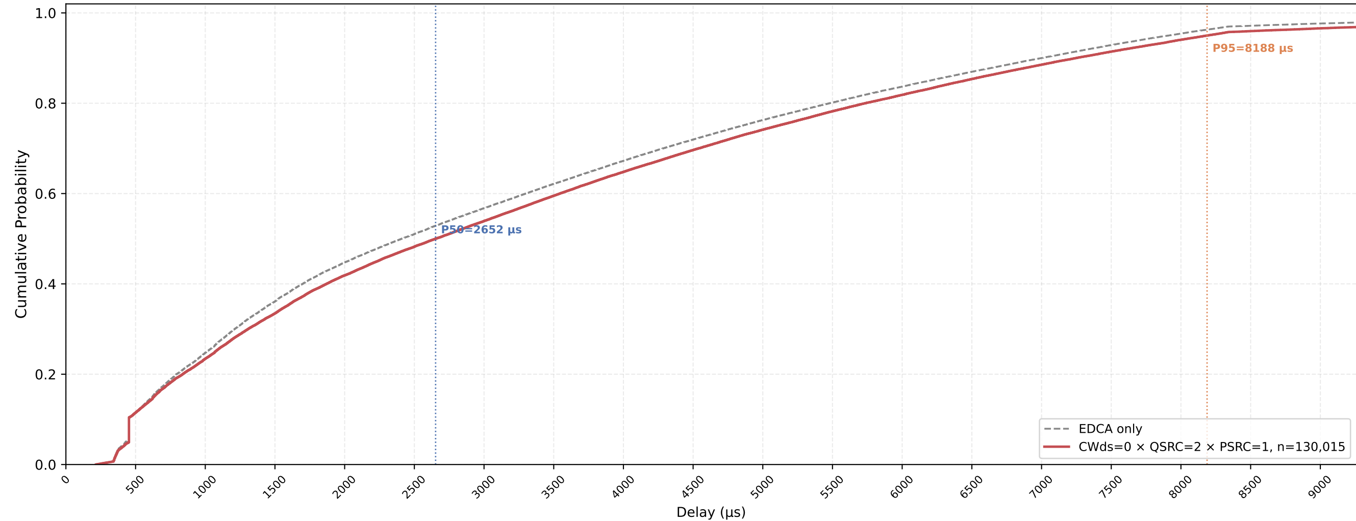
Legacy STA VO Delay CDF — CWds=0 × QSRC=2 × PSRC=1 nSta=30, nPedca=5, 1Mbps, avg of 10 runs
