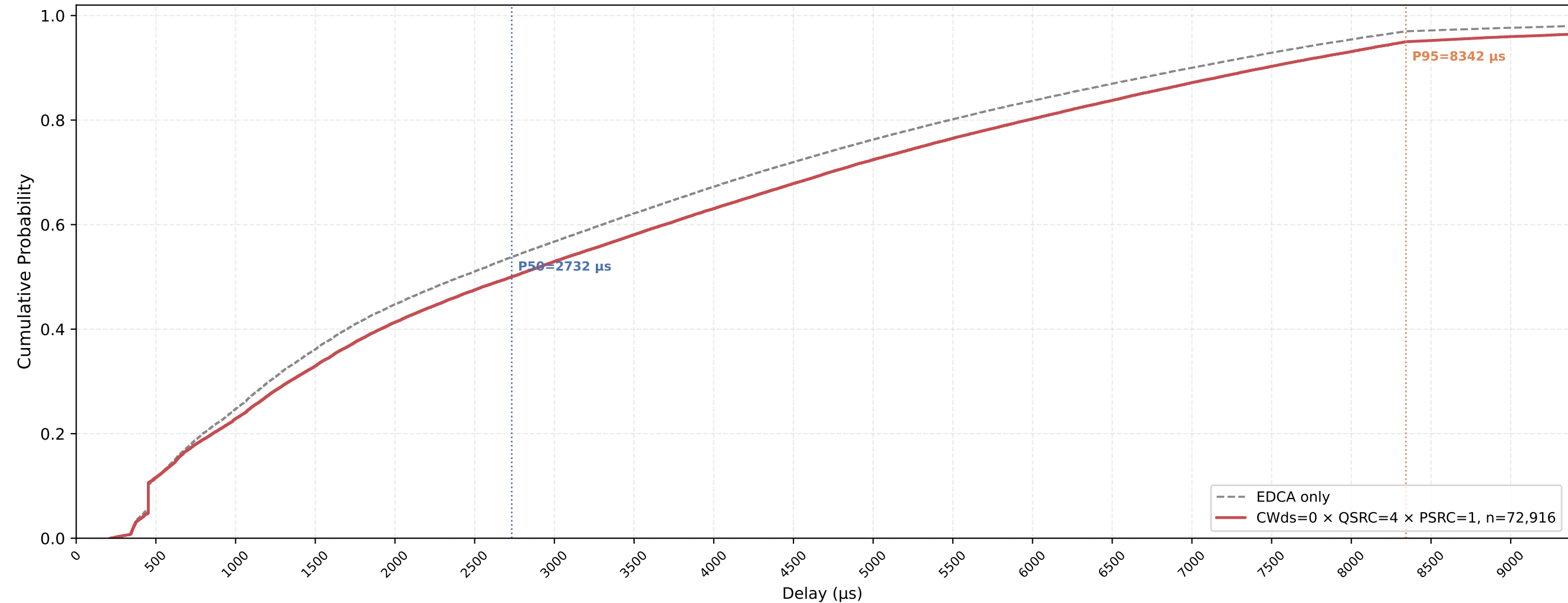
Legacy STA VO Delay CDF — CWds=0 × QSRC=4 × PSRC=1 nSta=30, nPedca=15, 1Mbps, avg of 10 runs
