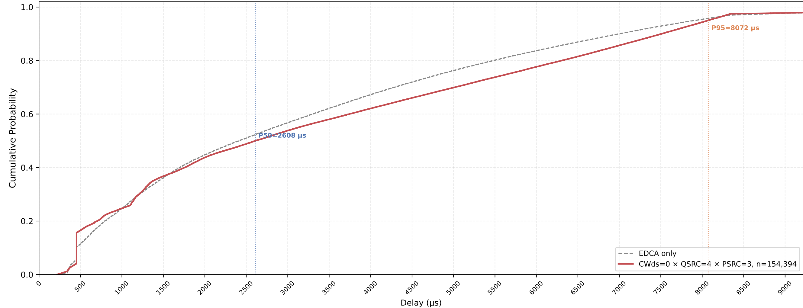
P-EDCA STA VO Delay CDF — CWds=0 × QSRC=4 × PSRC=3 nSta=30, nPedca=30, 1Mbps, avg of 10 runs
