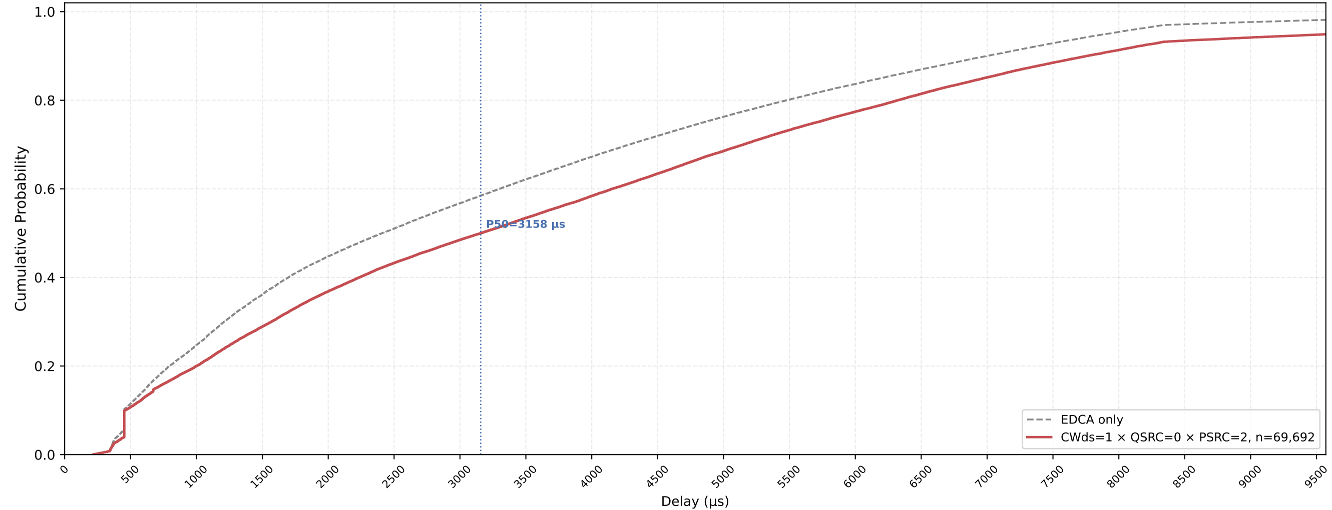
Legacy STA VO Delay CDF — CWds=1 × QSRC=0 × PSRC=2 nSta=30, nPedca=15, 1Mbps, avg of 10 runs
