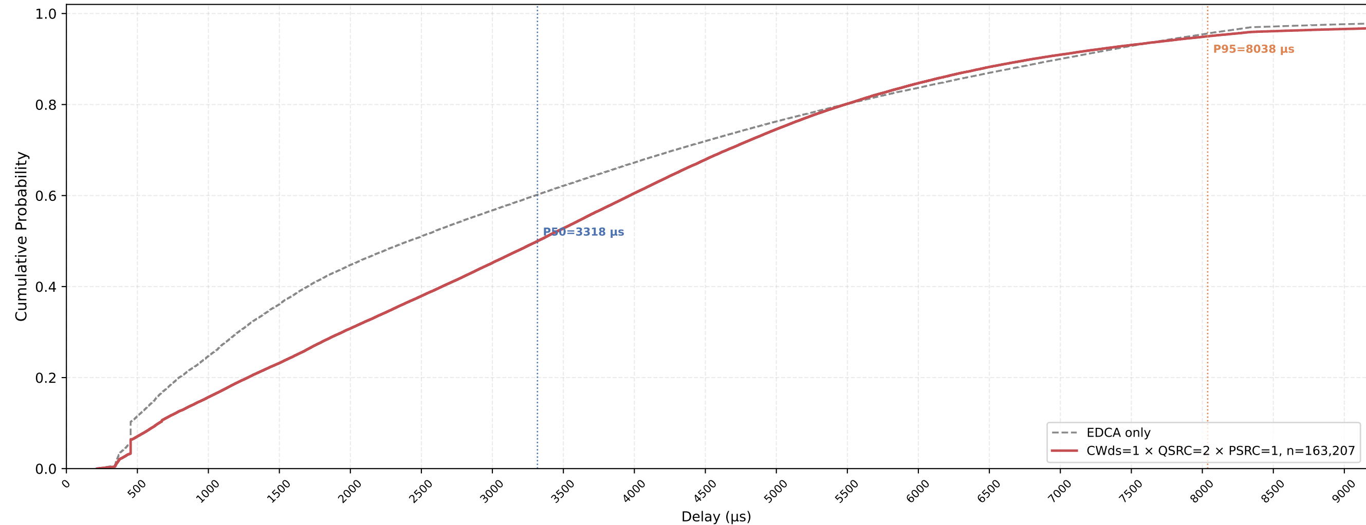
VO (all STAs) Delay CDF — CWds=1 × QSRC=2 × PSRC=1 nSta=30, nPedca=30, 1Mbps, avg of 10 runs
