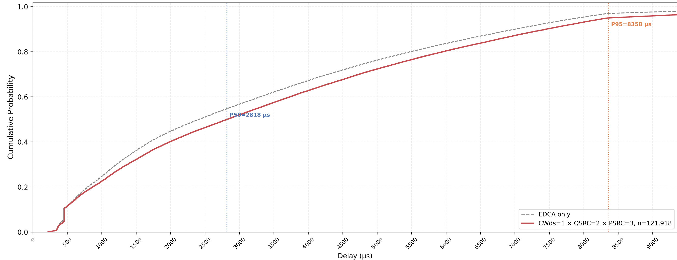
Legacy STA VO Delay CDF — CWds=1 × QSRC=2 × PSRC=3 nSta=30, nPedca=5, 1Mbps, avg of 10 runs
