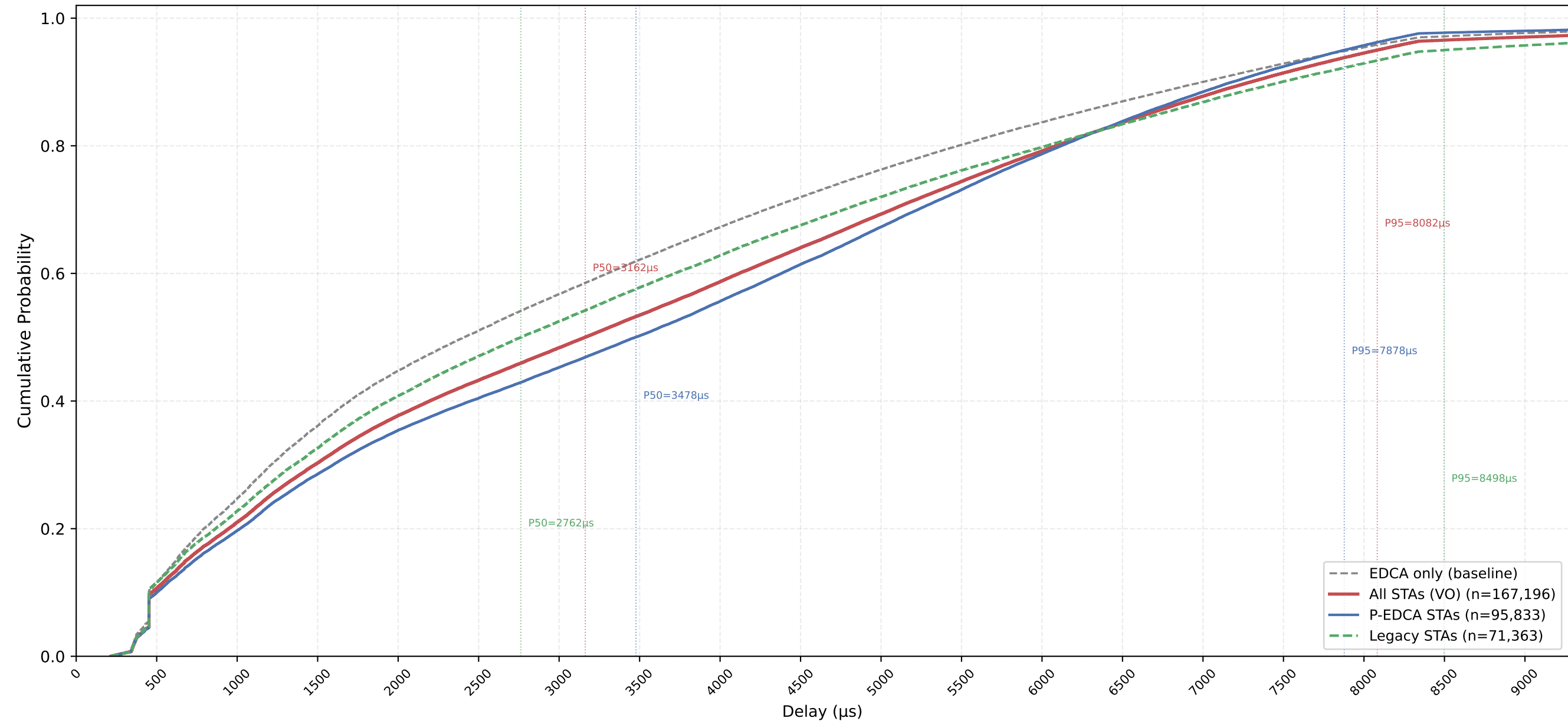
VO Delay CDF — P-EDCA / Legacy / All | CWds=1 × QSRC=3 × PSRC=1 nSta=30, nPedca=15/30, 1Mbps, avg of 10 runs
