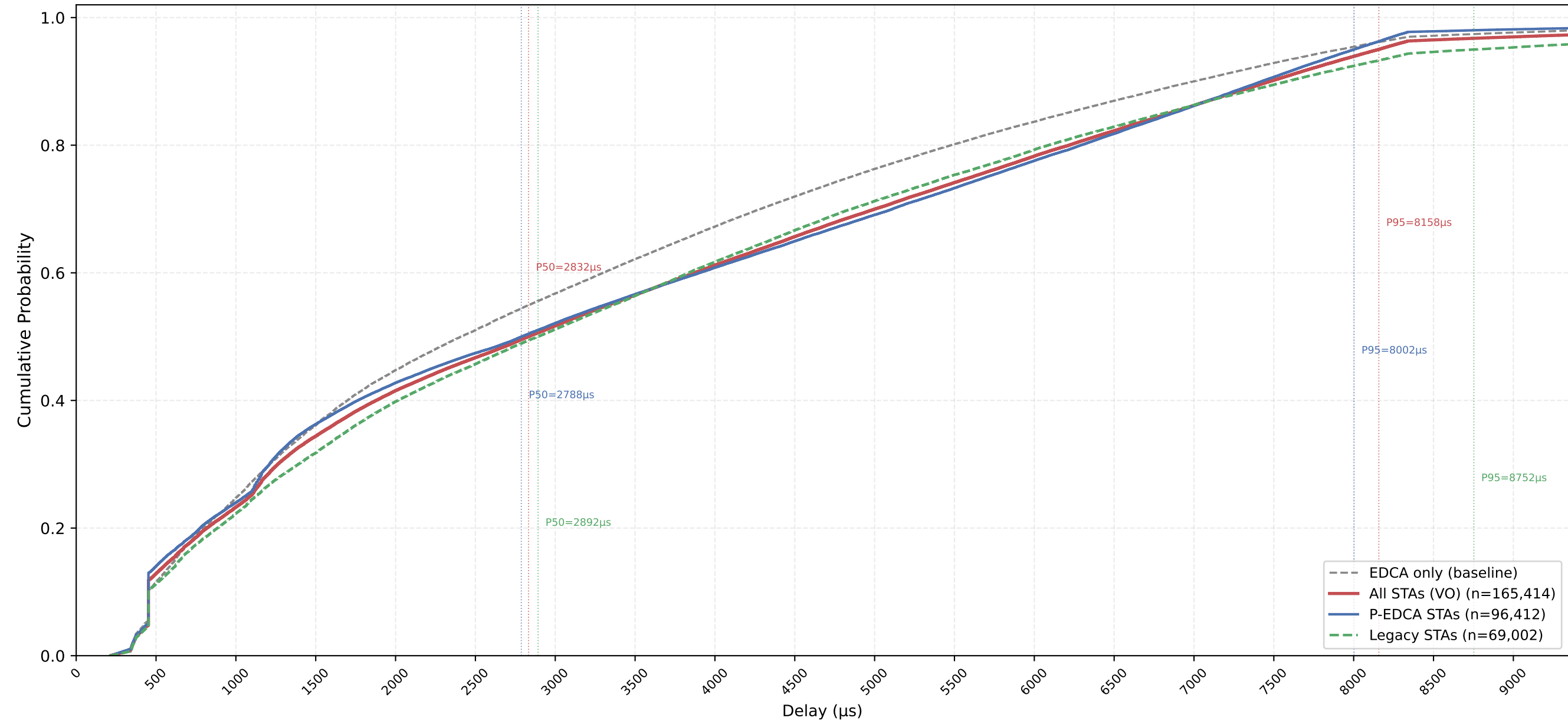
VO Delay CDF — P-EDCA / Legacy / All | CWds=1 × QSRC=4 × PSRC=1 nSta=30, nPedca=15/30, 1Mbps, avg of 10 runs
