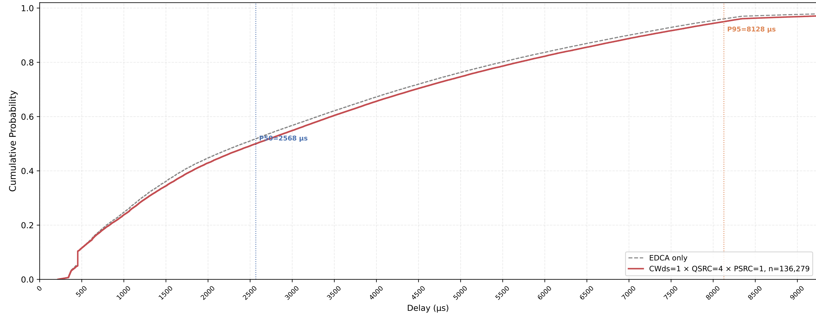
Legacy STA VO Delay CDF — CWds=1 × QSRC=4 × PSRC=1 nSta=30, nPedca=5, 1Mbps, avg of 10 runs
