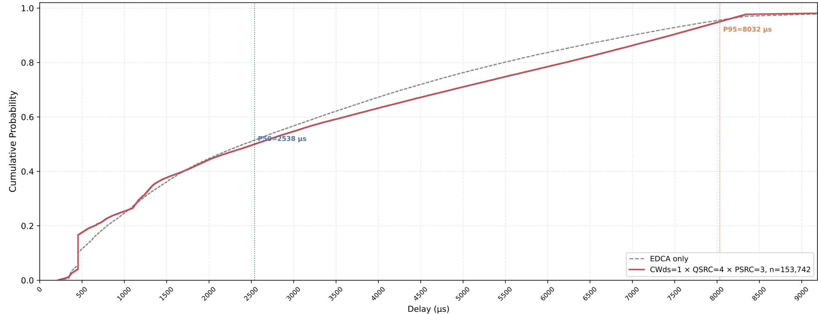
VO (all STAs) Delay CDF — CWds=1 × QSRC=4 × PSRC=3 nSta=30, nPedca=30, 1Mbps, avg of 10 runs
