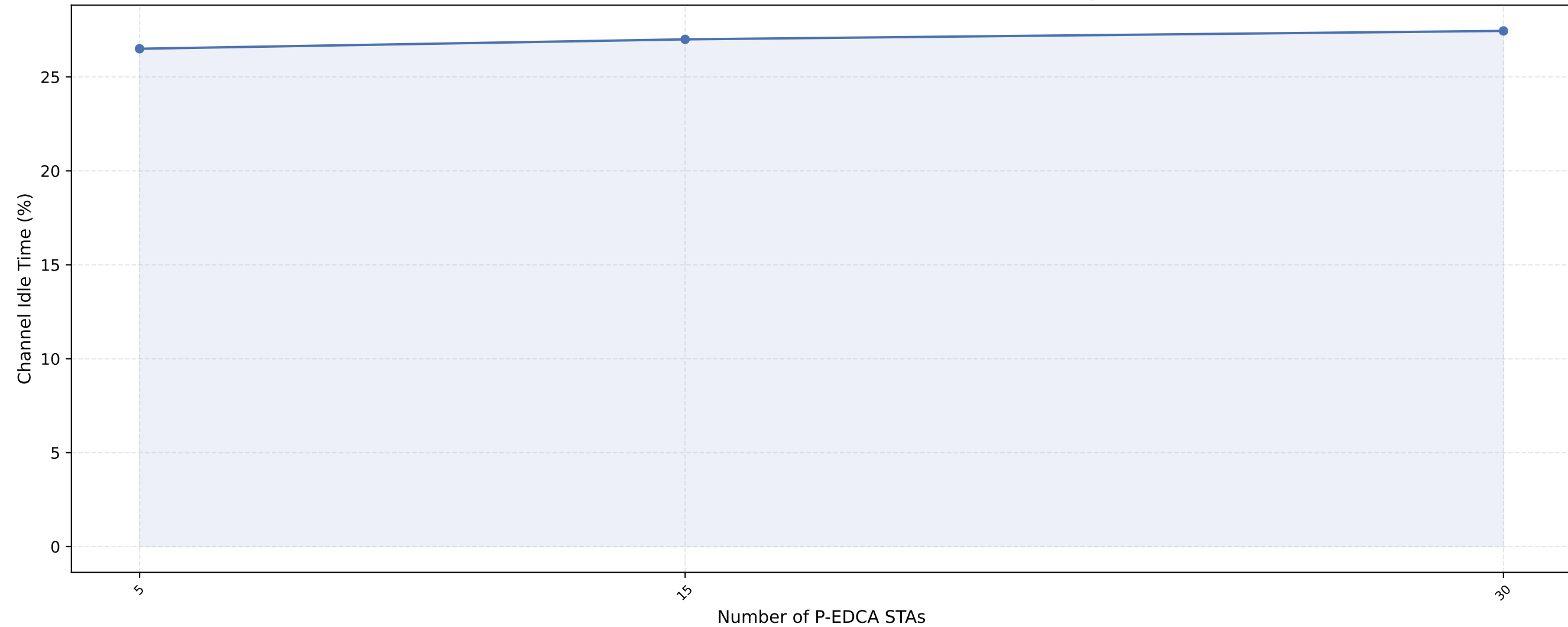
Channel Idle Time vs P-EDCA STAs — nSta=30, 1Mbps (avg of 10 runs)
