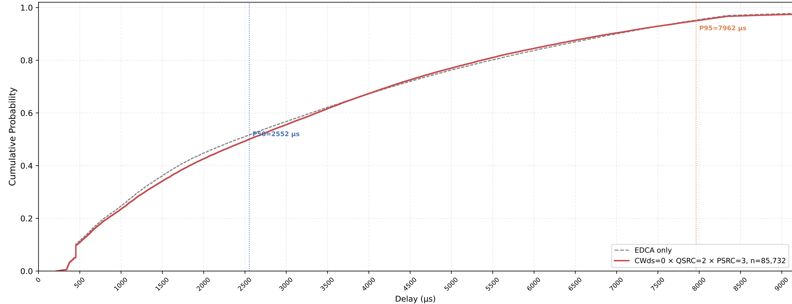
P-EDCA STA VO Delay CDF — CWds=0 × QSRC=2 × PSRC=3 nSta=30, nPedca=15, 1Mbps, avg of 10 runs
