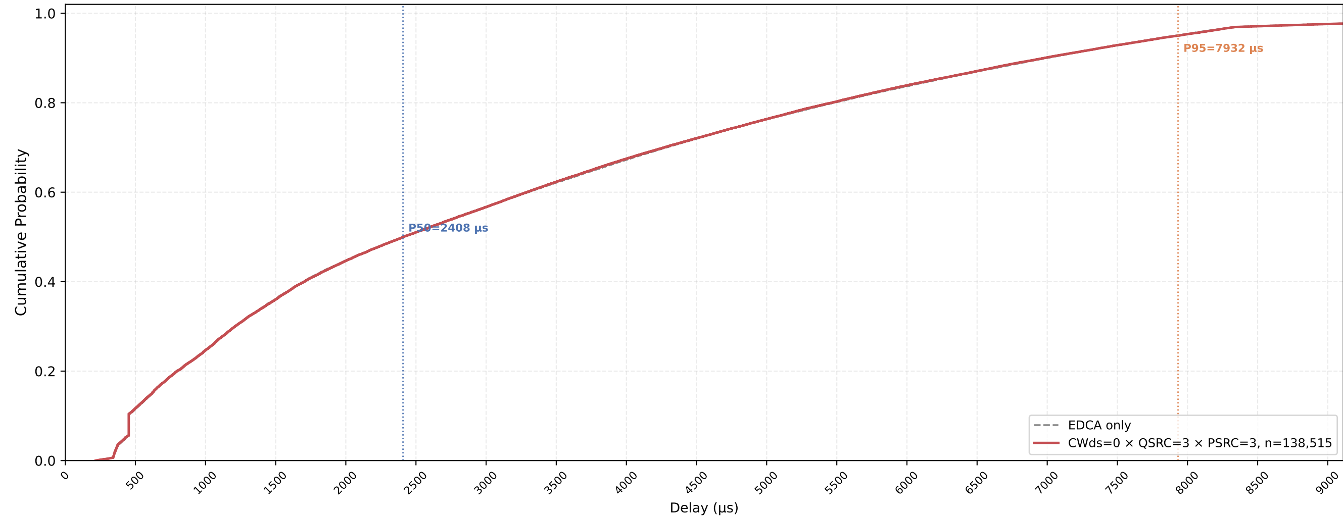
Legacy STA VO Delay CDF — CWds=0 × QSRC=3 × PSRC=3 nSta=30, nPedca=5, 1Mbps, avg of 10 runs
