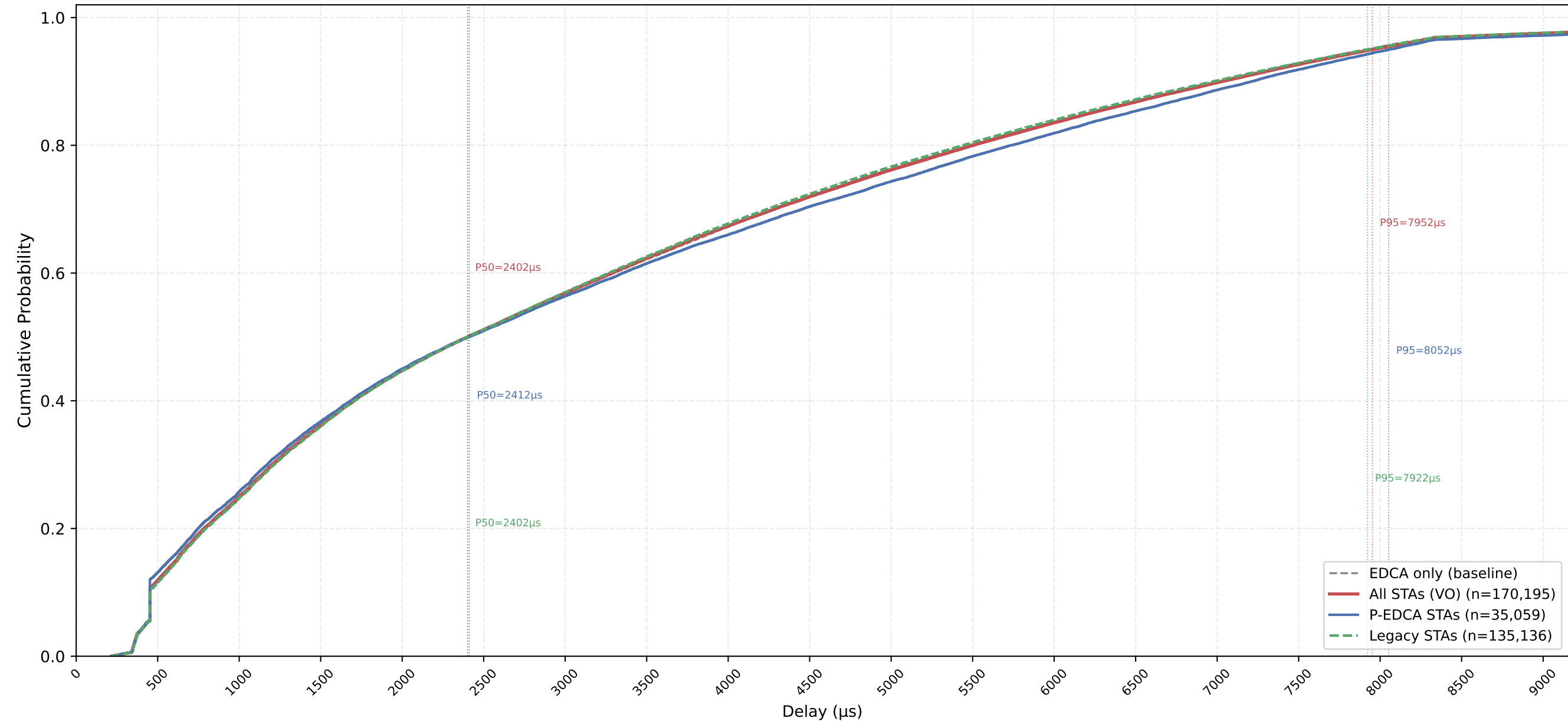
VO Delay CDF — P-EDCA / Legacy / All | CWds=0 × QSRC=4 × PSRC=3 nSta=30, nPedca=5/30, 1Mbps, avg of 10 runs
