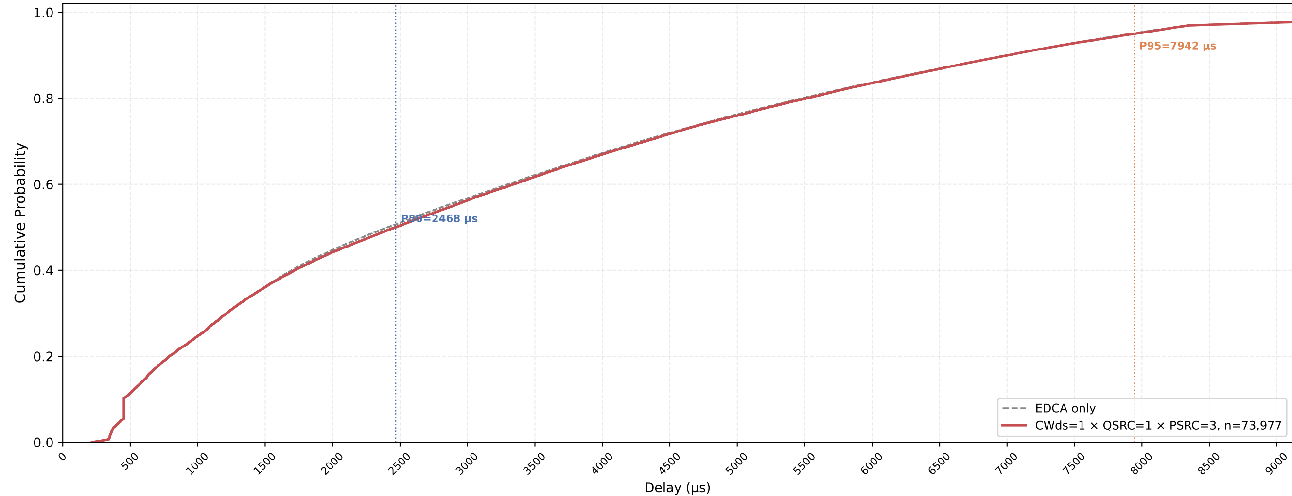
Legacy STA VO Delay CDF — CWds=1 × QSRC=1 × PSRC=3 nSta=30, nPedca=15, 1Mbps, avg of 10 runs
