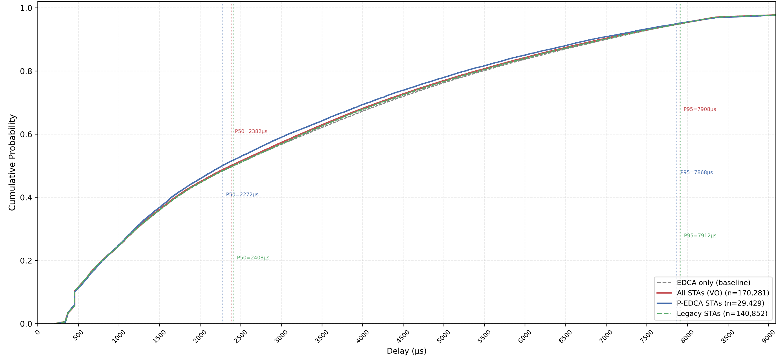
VO Delay CDF — P-EDCA / Legacy / All | CWds=1 × QSRC=2 × PSRC=2 nSta=30, nPedca=5/30, 1Mbps, avg of 10 runs
