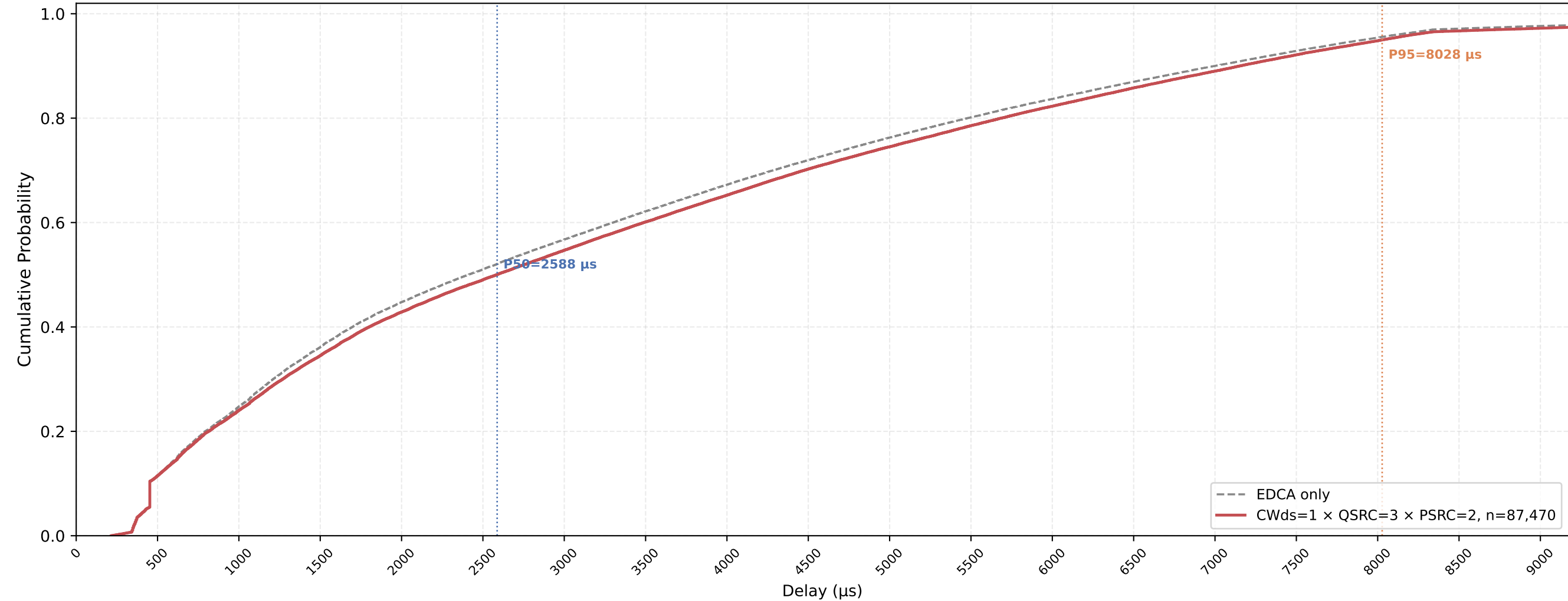
P-EDCA STA VO Delay CDF — CWds=1 × QSRC=3 × PSRC=2 nSta=30, nPedca=15, 1Mbps, avg of 10 runs
