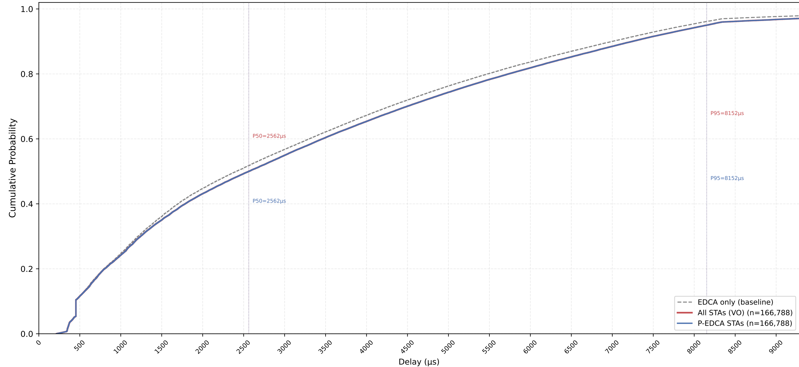
VO Delay CDF — P-EDCA / Legacy / All | CWds=1 × QSRC=5 × PSRC=1 nSta=30, nPedca=30/30, 1Mbps, avg of 10 runs
