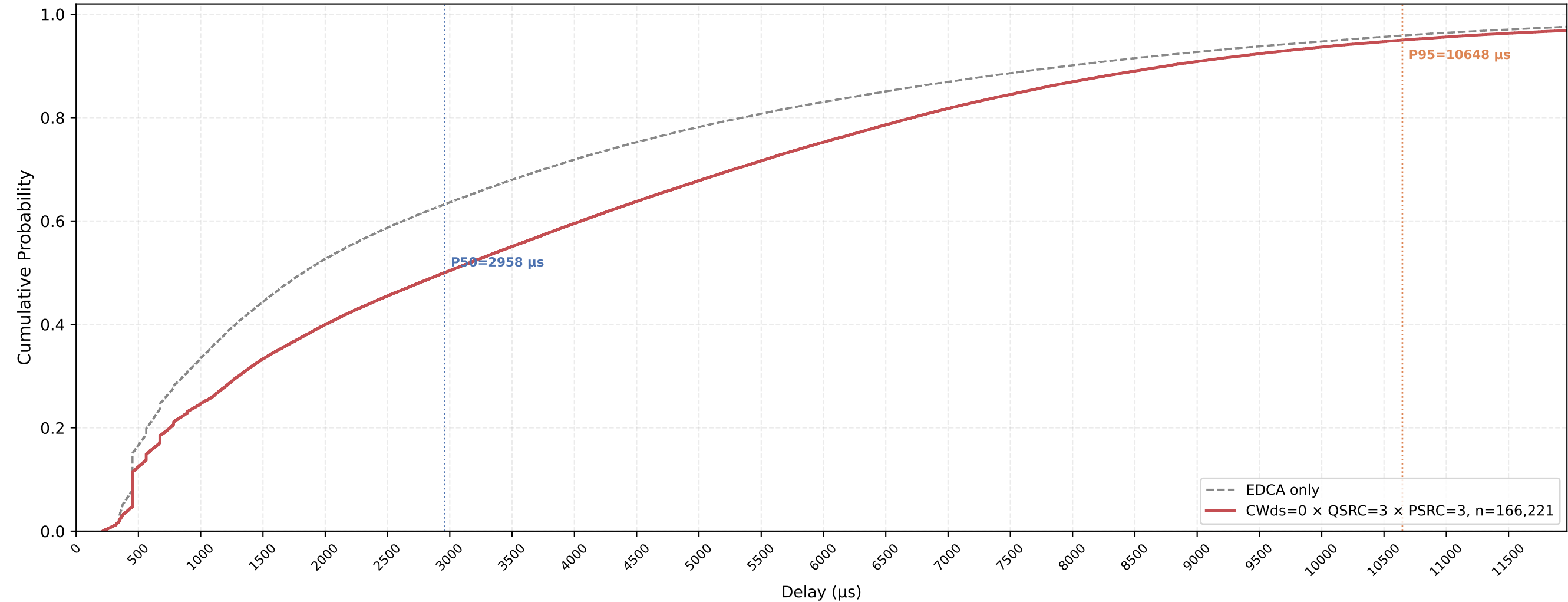
P-EDCA STA VO Delay CDF — CWds=0 × QSRC=3 × PSRC=3 nSta=30, nPedca=30, 1Mbps, avg of 10 runs
