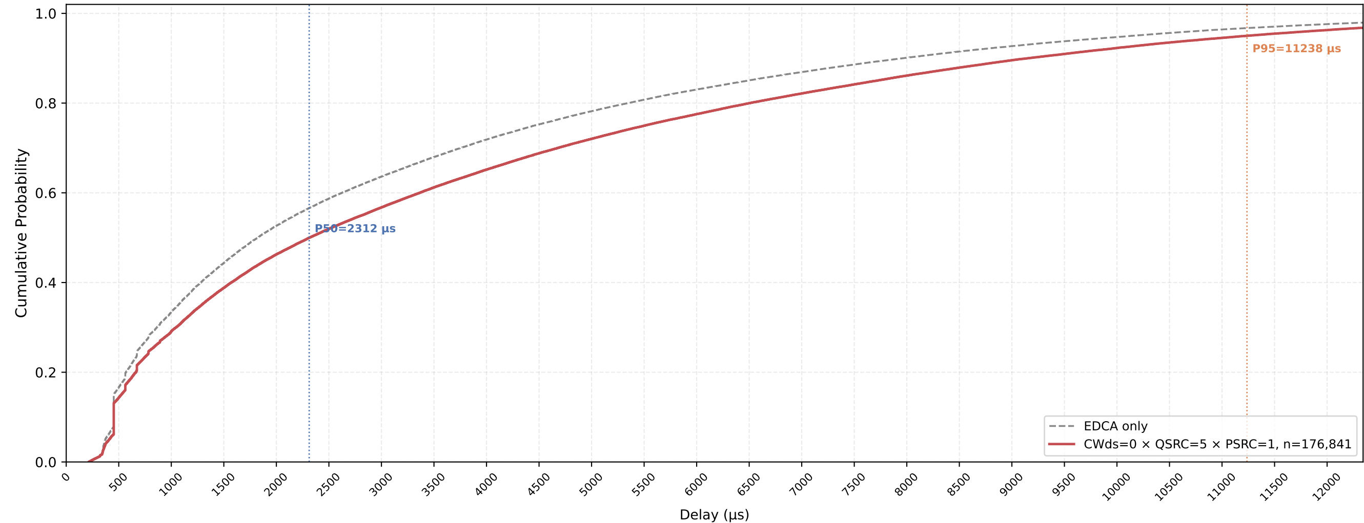
VO (all STAs) Delay CDF — CWds=0 × QSRC=5 × PSRC=1 nSta=30, nPedca=15, 1Mbps, avg of 10 runs
