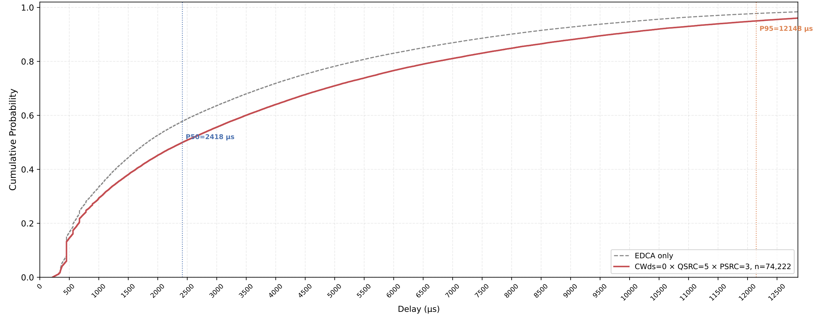
Legacy STA VO Delay CDF — CWds=0 × QSRC=5 × PSRC=3 nSta=30, nPedca=15, 1Mbps, avg of 10 runs
