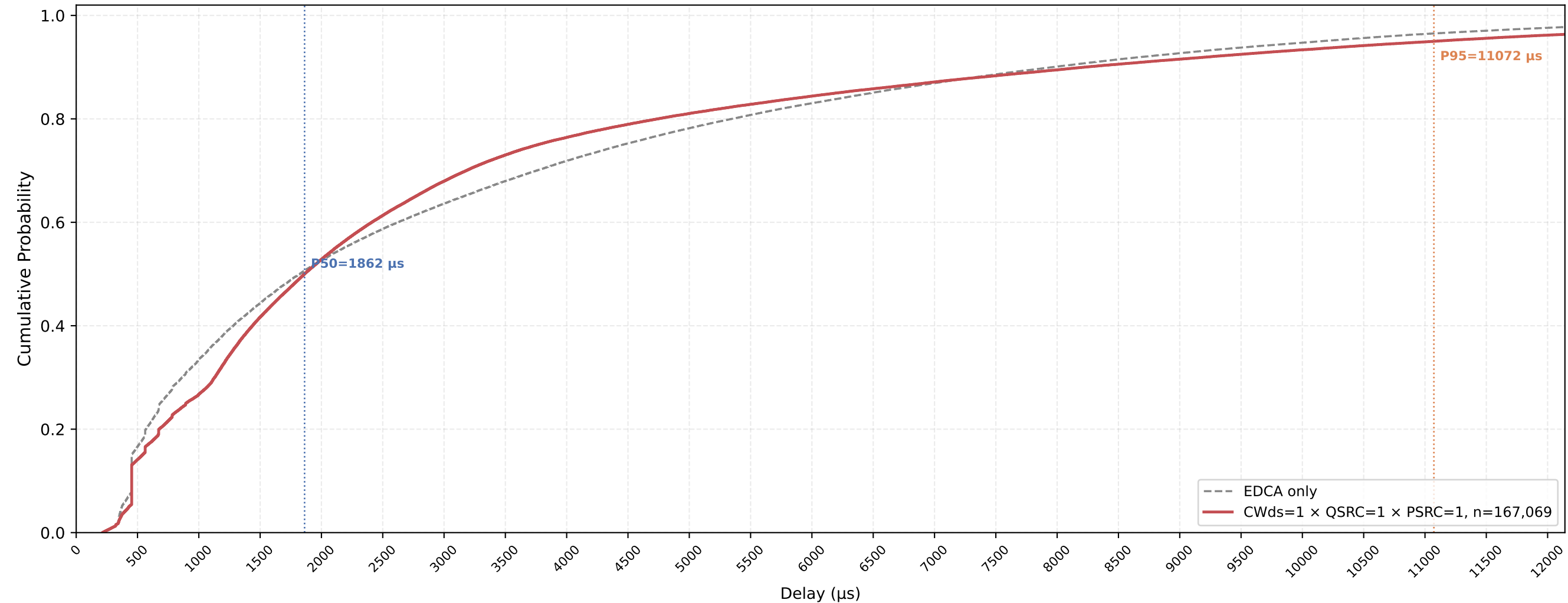
VO (all STAs) Delay CDF — CWds=1 × QSRC=1 × PSRC=1 nSta=30, nPedca=30, 1Mbps, avg of 10 runs
