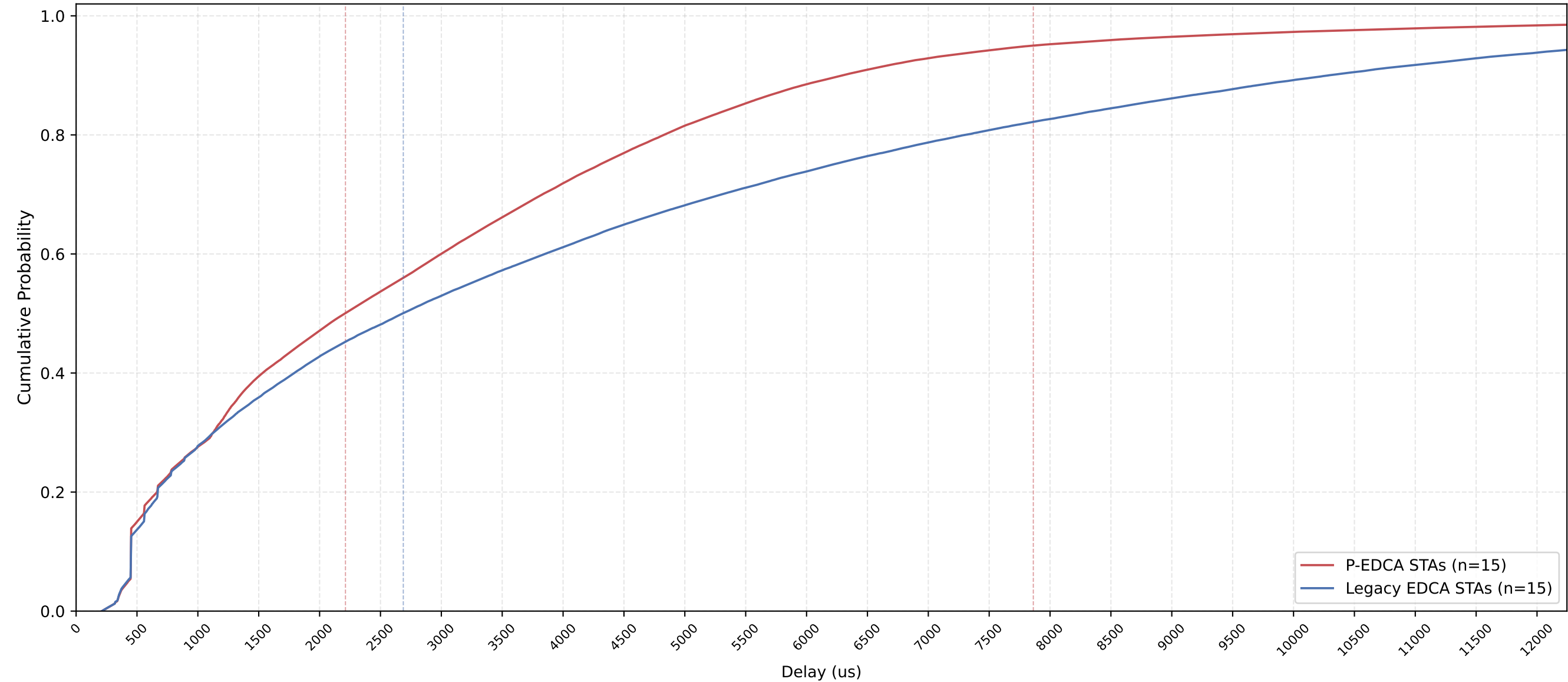
P-EDCA vs Legacy Delay CDF — n_pedca=15, n_legacy=15, nSta=30, 1Mbps, avg of 10 runs
