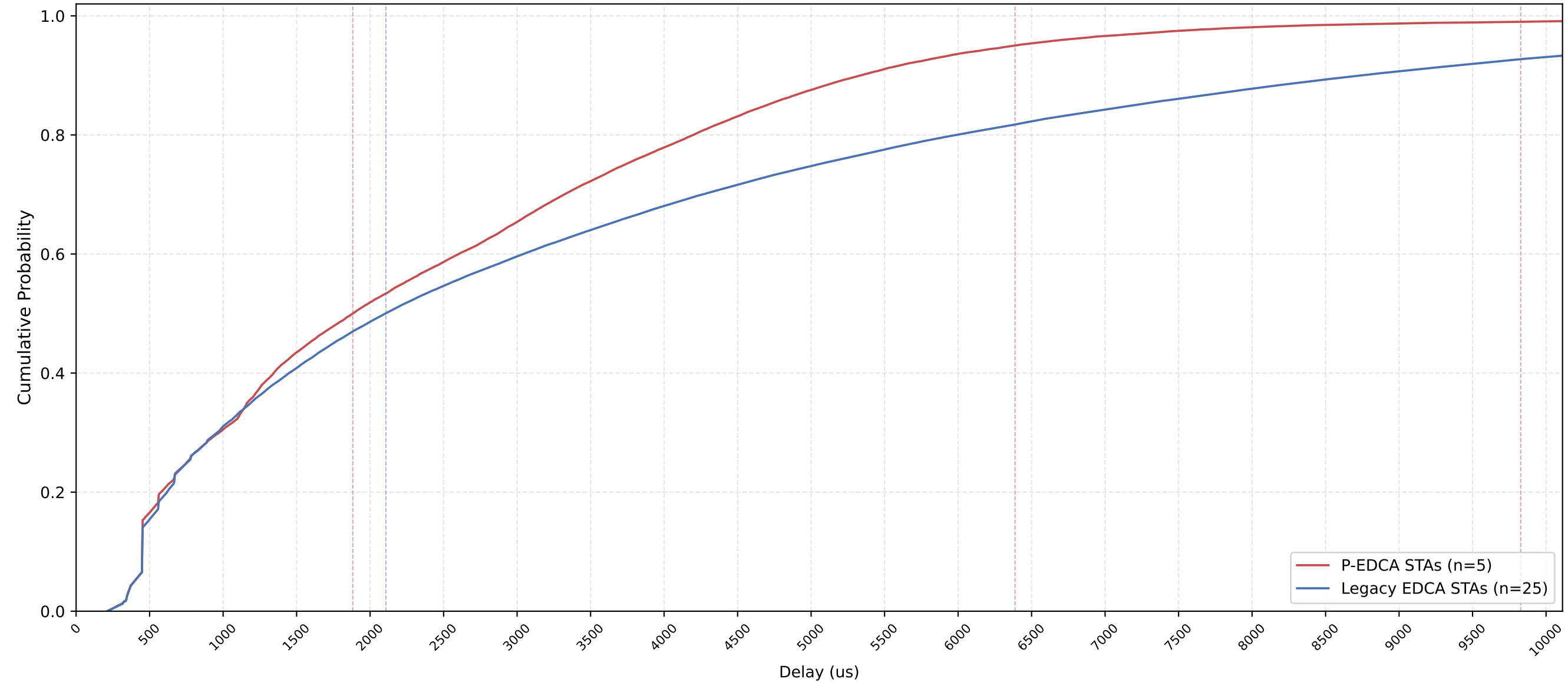
P-EDCA vs Legacy Delay CDF — n_pedca=5, n_legacy=25, nSta=30, 1Mbps, avg of 10 runs
