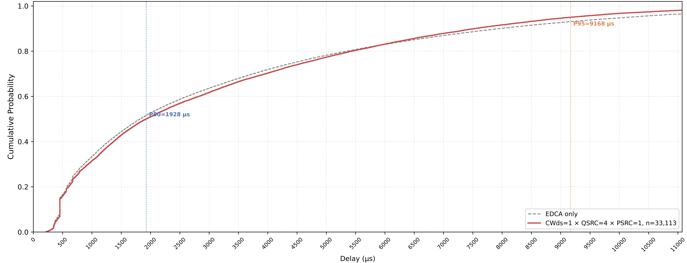
P-EDCA STA VO Delay CDF — CWds=1 × QSRC=4 × PSRC=1 nSta=30, nPedca=5, 1Mbps, avg of 10 runs
