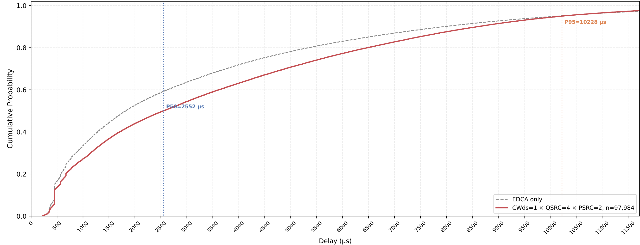
P-EDCA STA VO Delay CDF — CWds=1 × QSRC=4 × PSRC=2 nSta=30, nPedca=15, 1Mbps, avg of 10 runs
