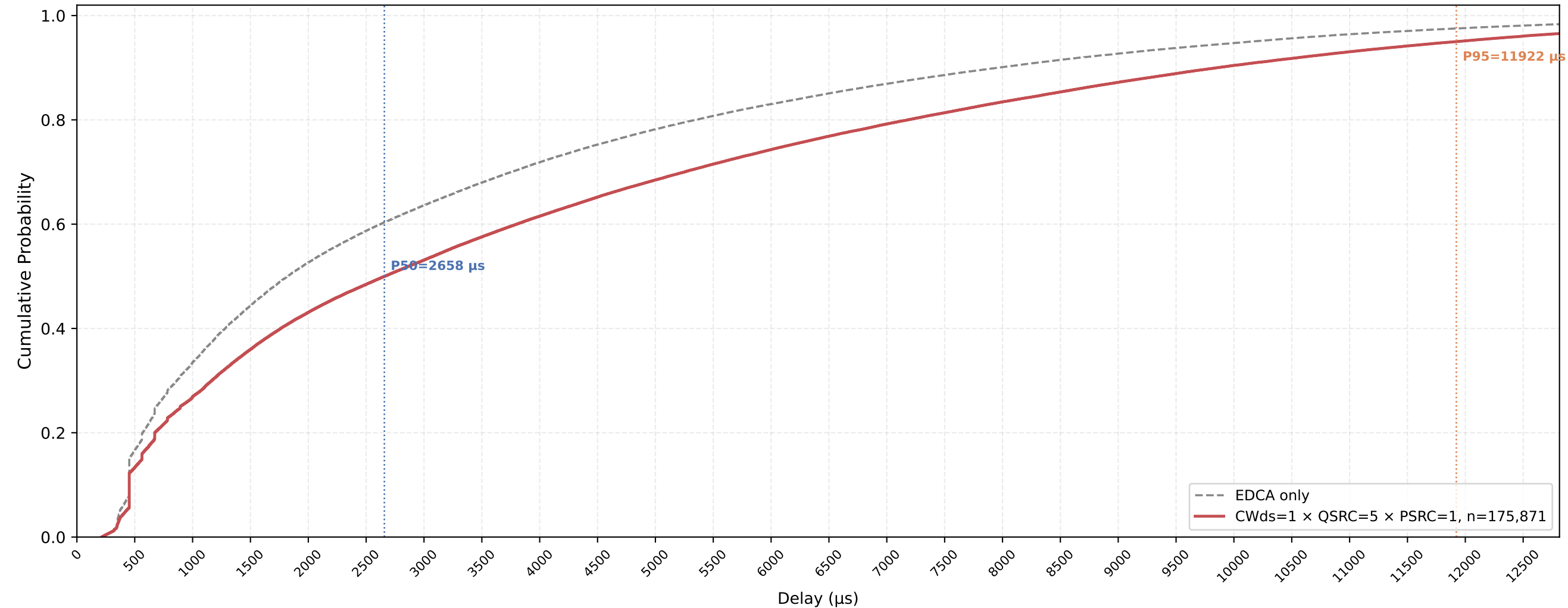
VO (all STAs) Delay CDF — CWds=1 × QSRC=5 × PSRC=1 nSta=30, nPedca=30, 1Mbps, avg of 10 runs
