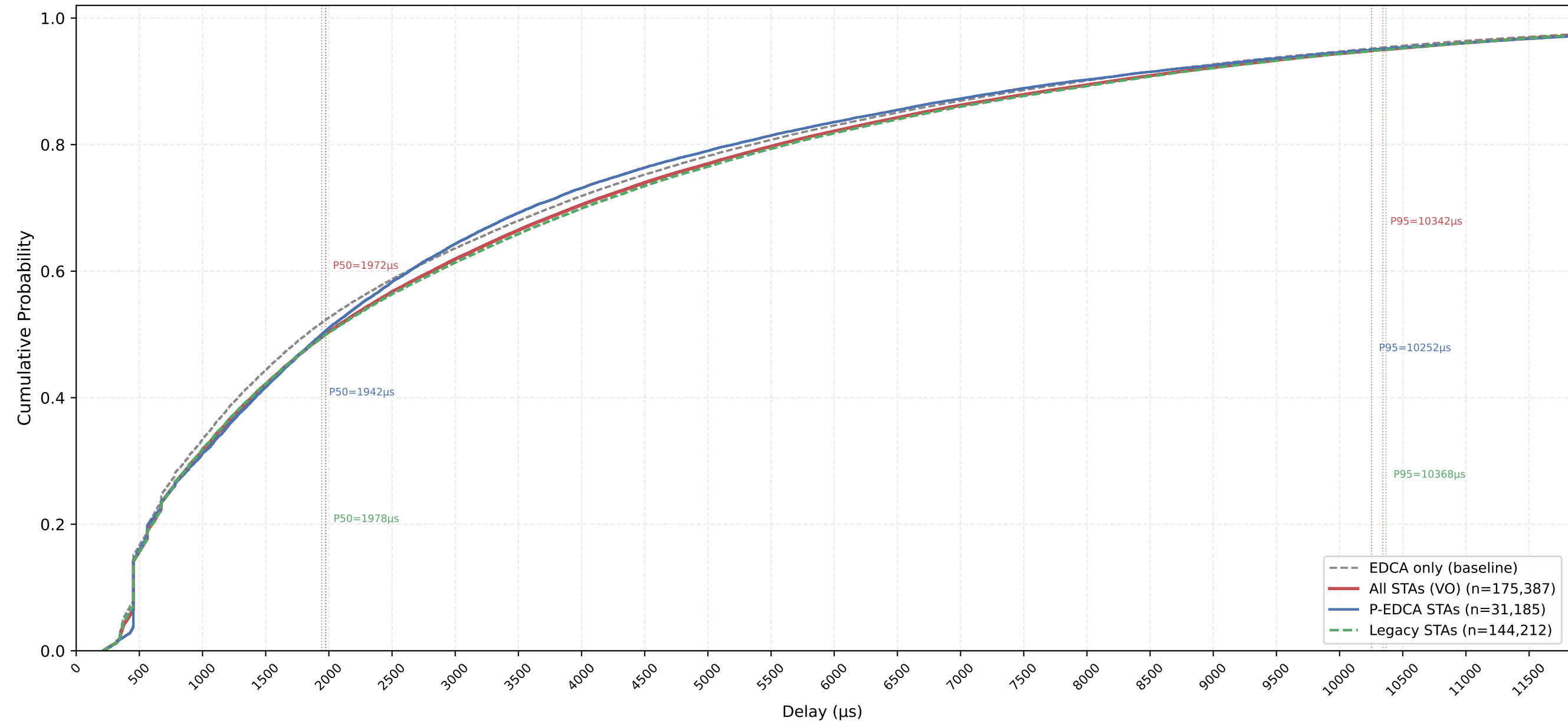
VO Delay CDF — P-EDCA / Legacy / All | CWds=0 × QSRC=0 × PSRC=3 nSta=30, nPedca=5/30, 1Mbps, avg of 10 runs
