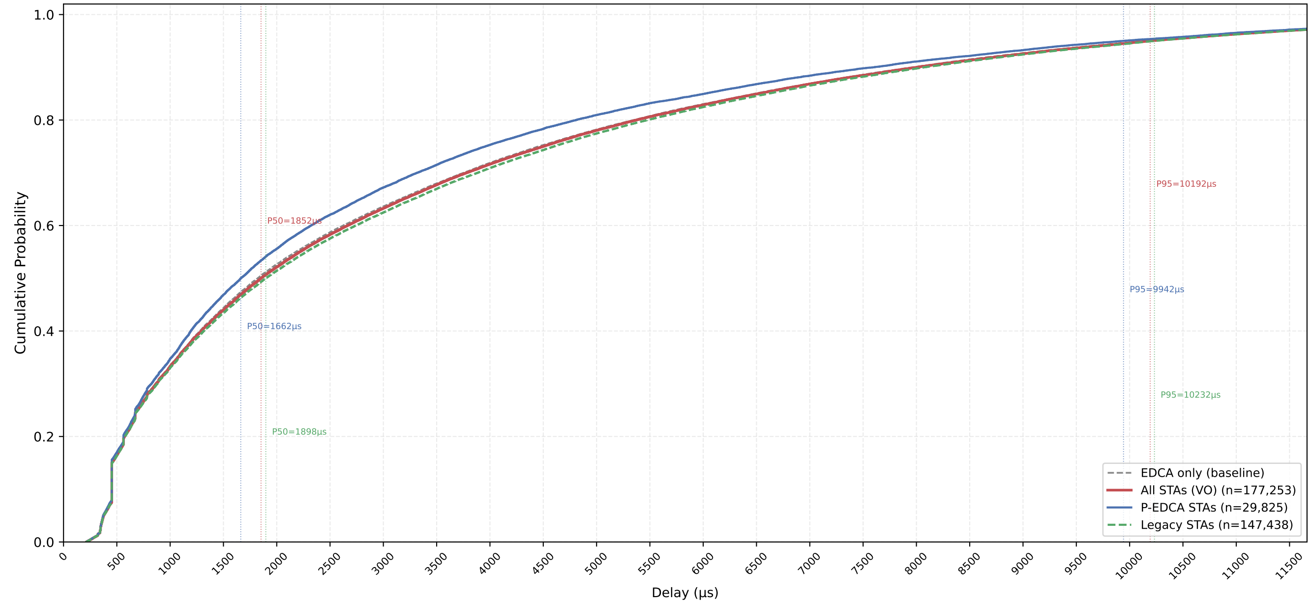
VO Delay CDF — P-EDCA / Legacy / All | CWds=0 × QSRC=1 × PSRC=2 nSta=30, nPedca=5/30, 1Mbps, avg of 10 runs
