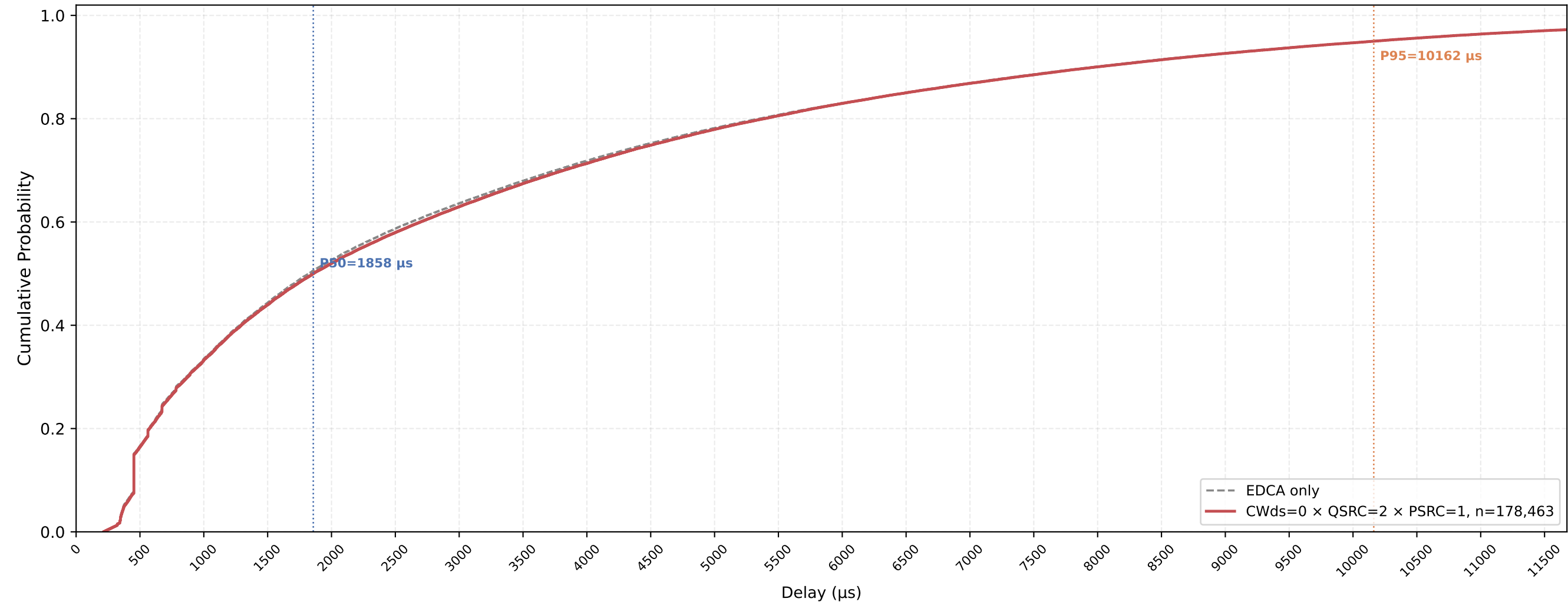
VO (all STAs) Delay CDF — CWds=0 × QSRC=2 × PSRC=1 nSta=30, nPedca=5, 1Mbps, avg of 10 runs
