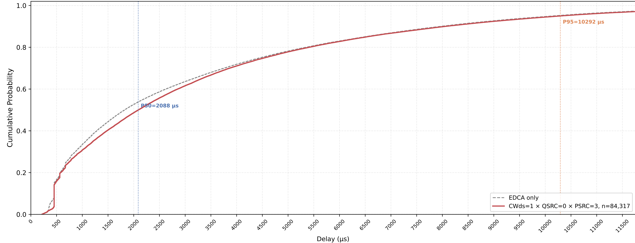
P-EDCA STA VO Delay CDF — CWds=1 × QSRC=0 × PSRC=3 nSta=30, nPedca=15, 1Mbps, avg of 10 runs
