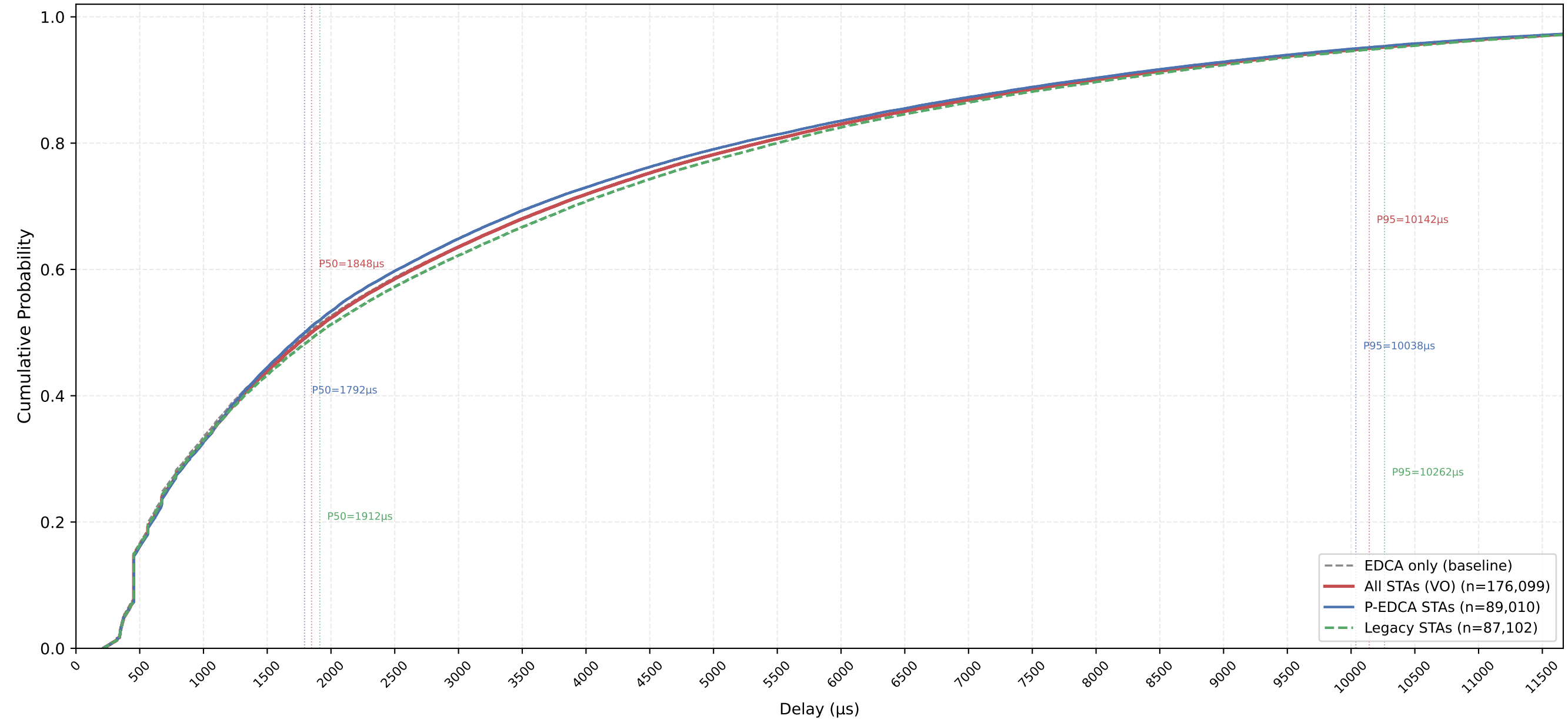
VO Delay CDF — P-EDCA / Legacy / All | CWds=1 × QSRC=1 × PSRC=1 nSta=30, nPedca=15/30, 1Mbps, avg of 10 runs
