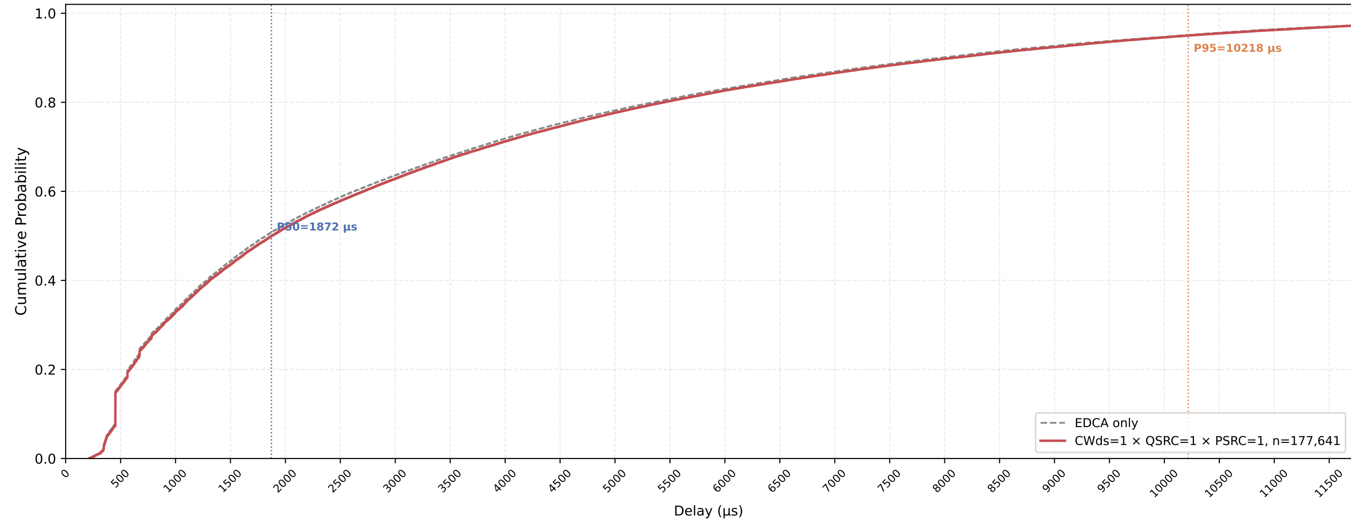
VO (all STAs) Delay CDF — CWds=1 × QSRC=1 × PSRC=1 nSta=30, nPedca=5, 1Mbps, avg of 10 runs
