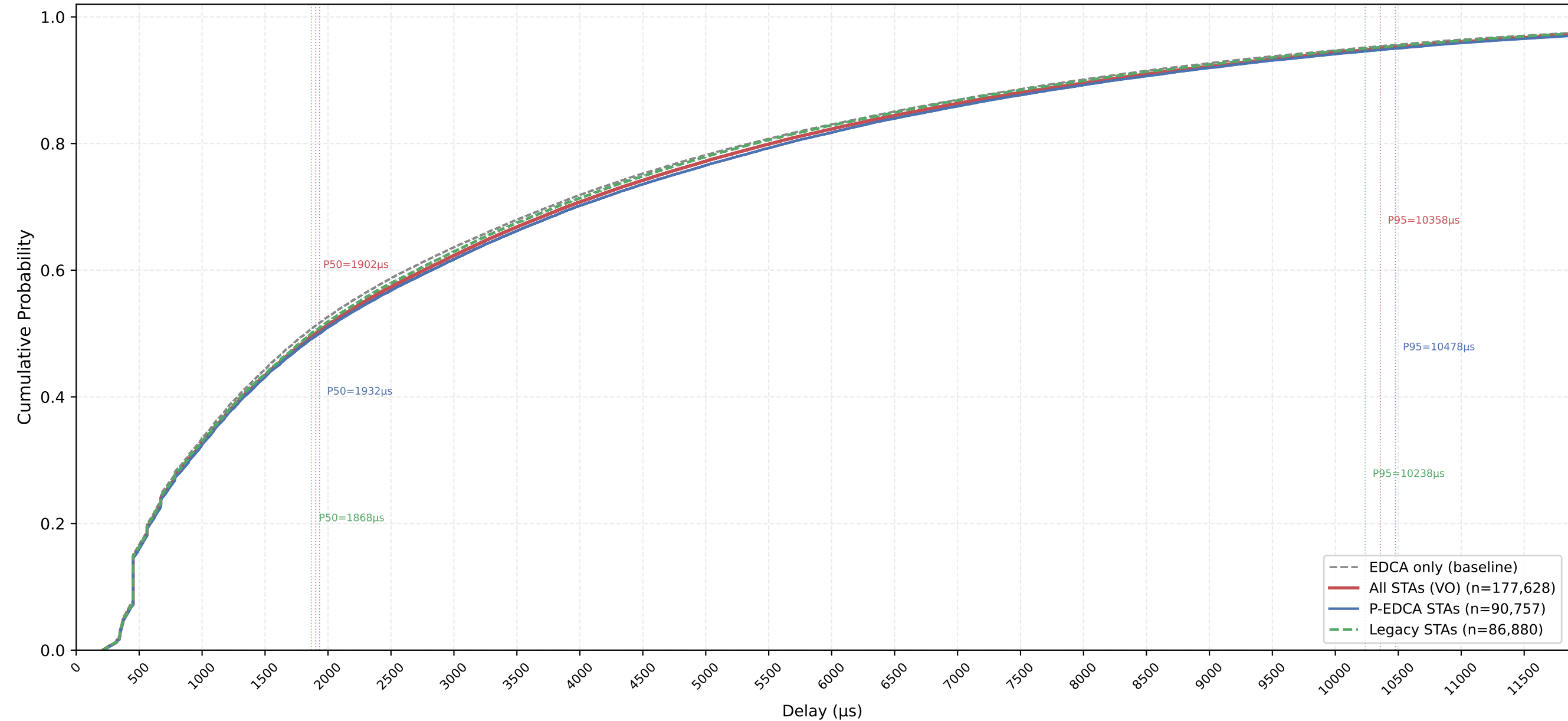
VO Delay CDF — P-EDCA / Legacy / All | CWds=1 × QSRC=4 × PSRC=2 nSta=30, nPedca=15/30, 1Mbps, avg of 10 runs
