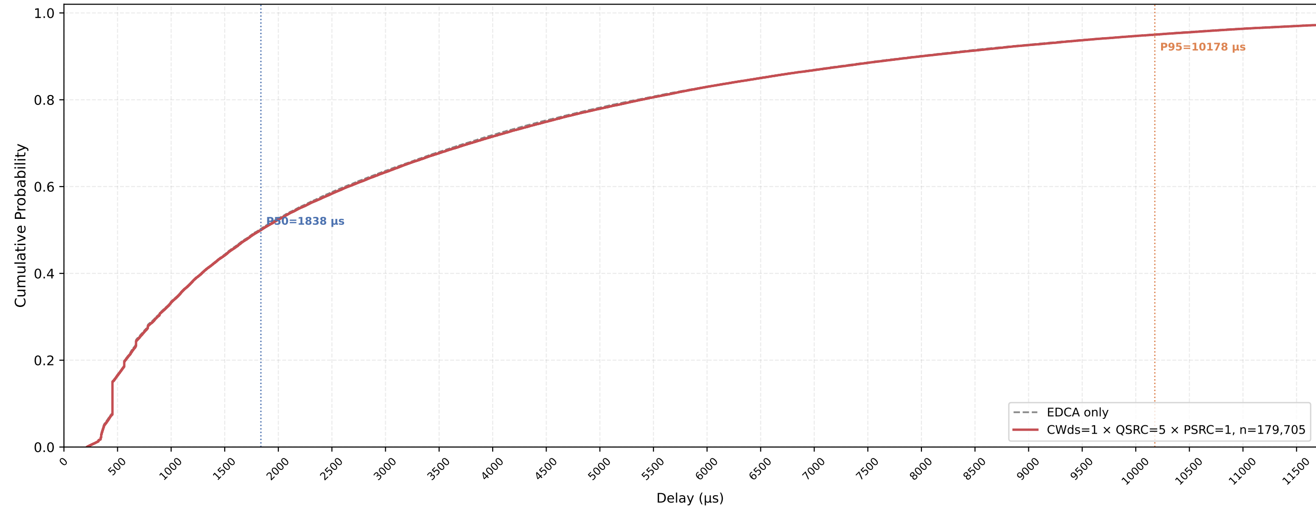
VO (all STAs) Delay CDF — CWds=1 × QSRC=5 × PSRC=1 nSta=30, nPedca=5, 1Mbps, avg of 10 runs
