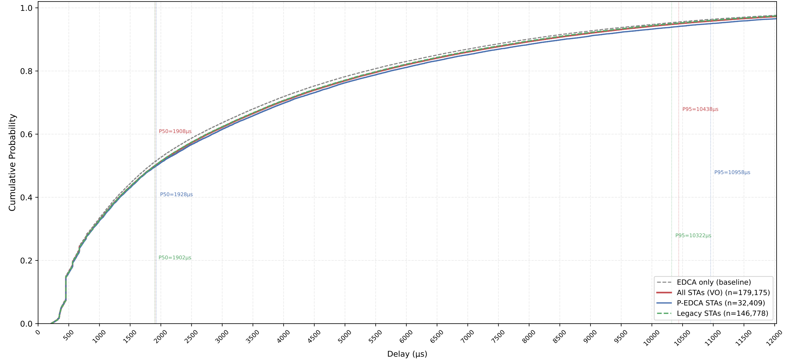
VO Delay CDF — P-EDCA / Legacy / All | CWds=1 × QSRC=5 × PSRC=3 nSta=30, nPedca=5/30, 1Mbps, avg of 10 runs
