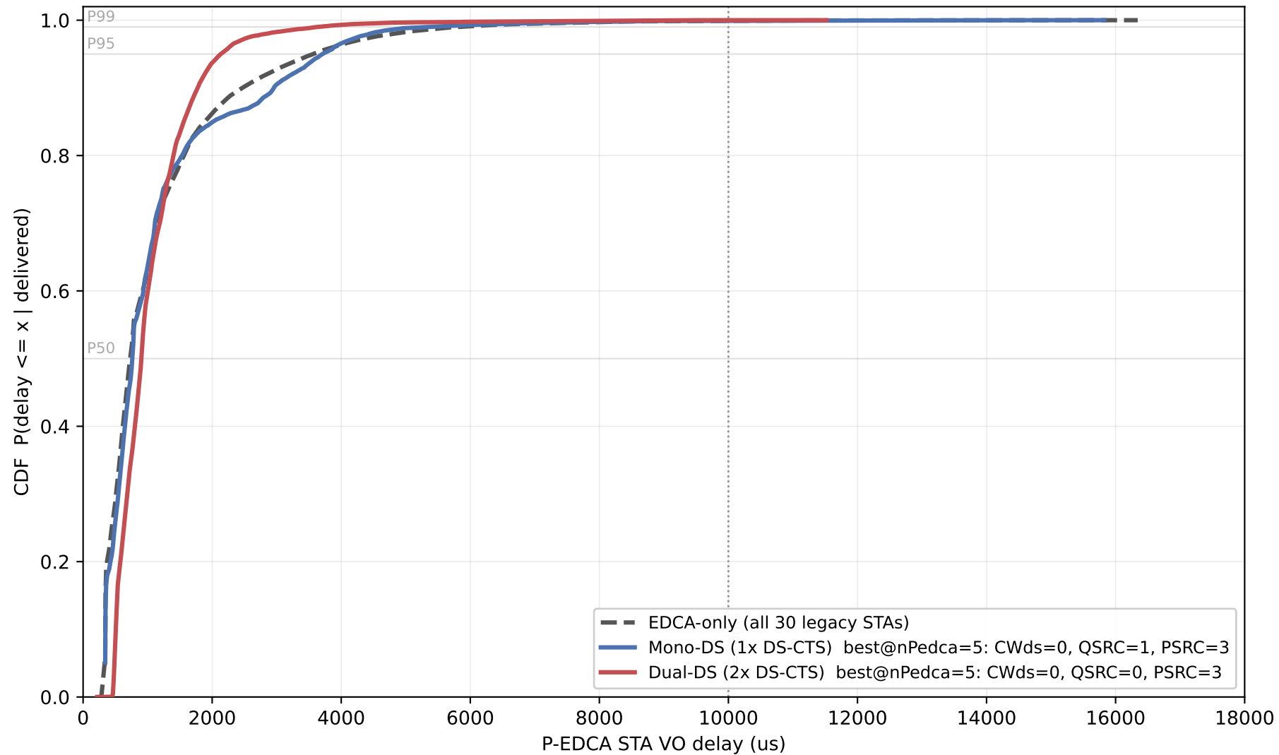
P-EDCA STA Delay CDF at Best Parameters (nPedca=5/30, nSta=30, 0.5Mbps) curves normalised to 1.0 — delay SHAPE only, loss not shown
