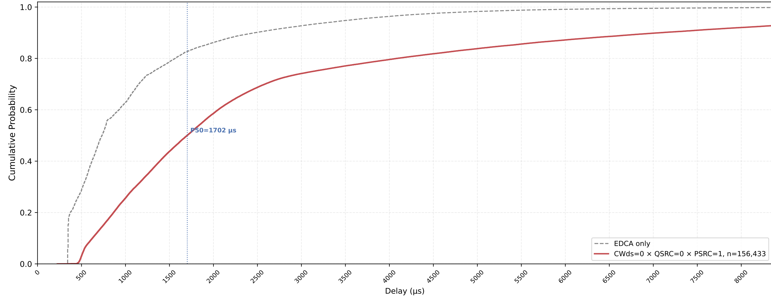
P-EDCA STA VO Delay CDF — CWds=0 × QSRC=0 × PSRC=1 nSta=30, nPedca=30, 0.5Mbps, avg of 10 runs
