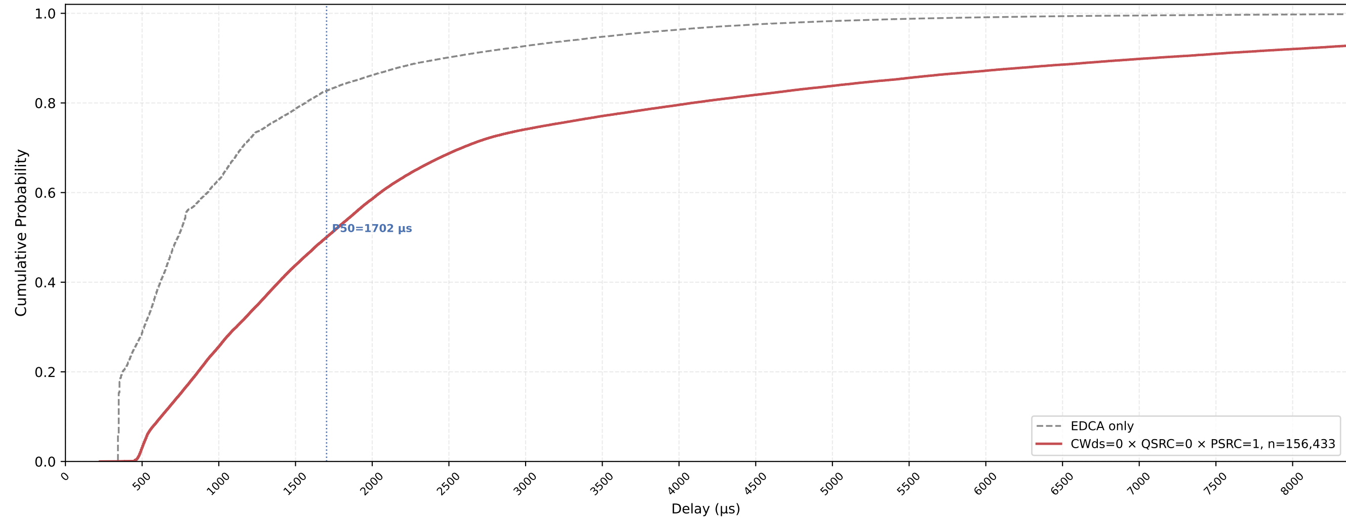
VO (all STAs) Delay CDF — CWds=0 × QSRC=0 × PSRC=1 nSta=30, nPedca=30, 0.5Mbps, avg of 10 runs
