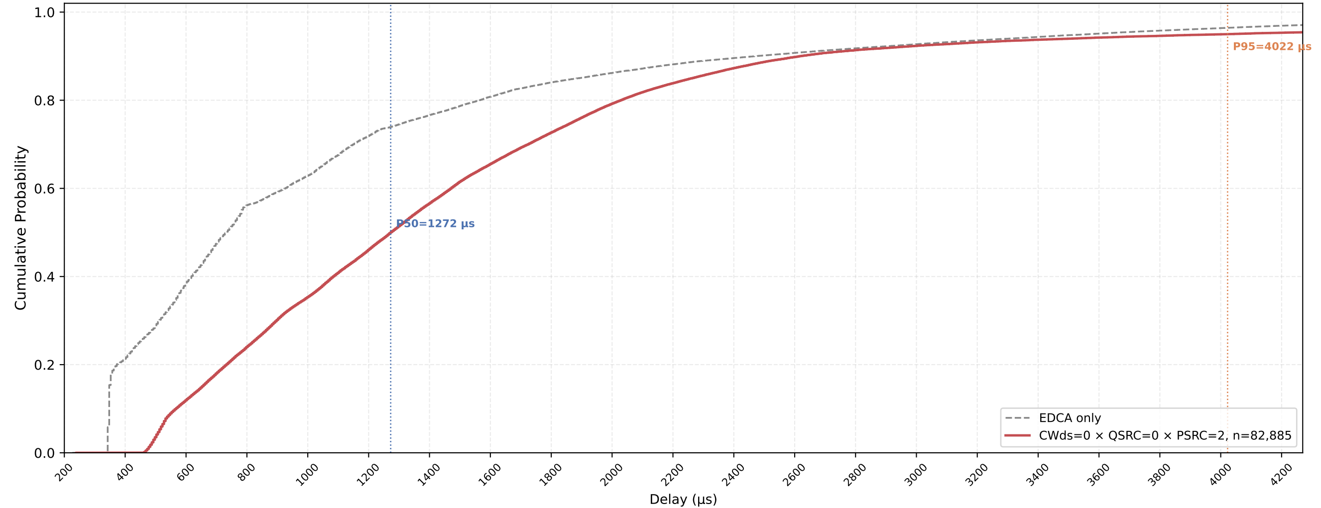
P-EDCA STA VO Delay CDF — CWds=0 × QSRC=0 × PSRC=2 nSta=30, nPedca=15, 0.5Mbps, avg of 10 runs
