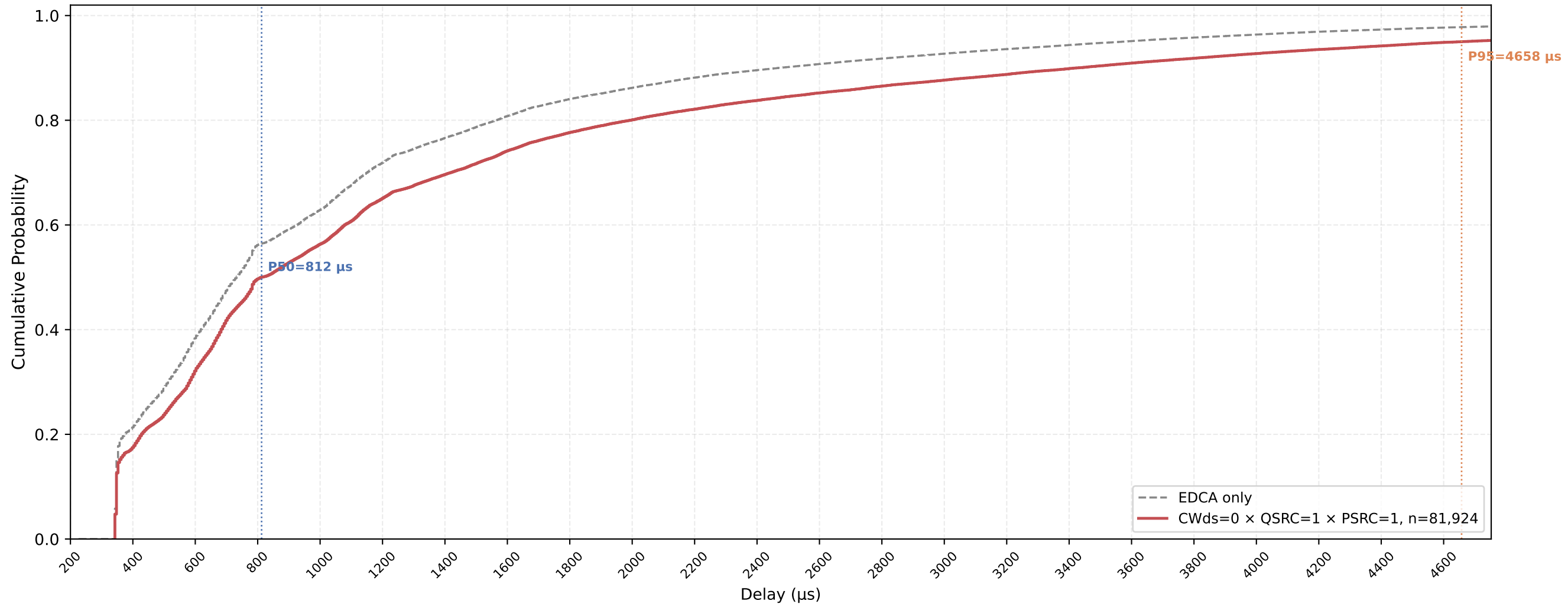
Legacy STA VO Delay CDF — CWds=0 × QSRC=1 × PSRC=1 nSta=30, nPedca=15, 0.5Mbps, avg of 10 runs
