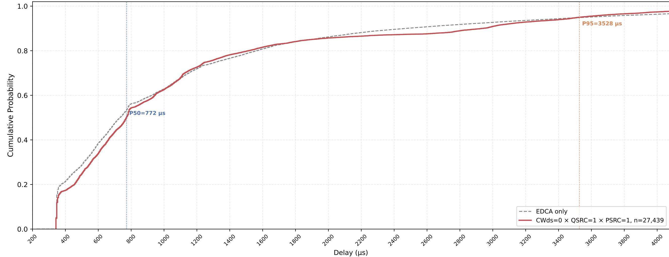
P-EDCA STA VO Delay CDF — CWds=0 × QSRC=1 × PSRC=1 nSta=30, nPedca=5, 0.5Mbps, avg of 10 runs
