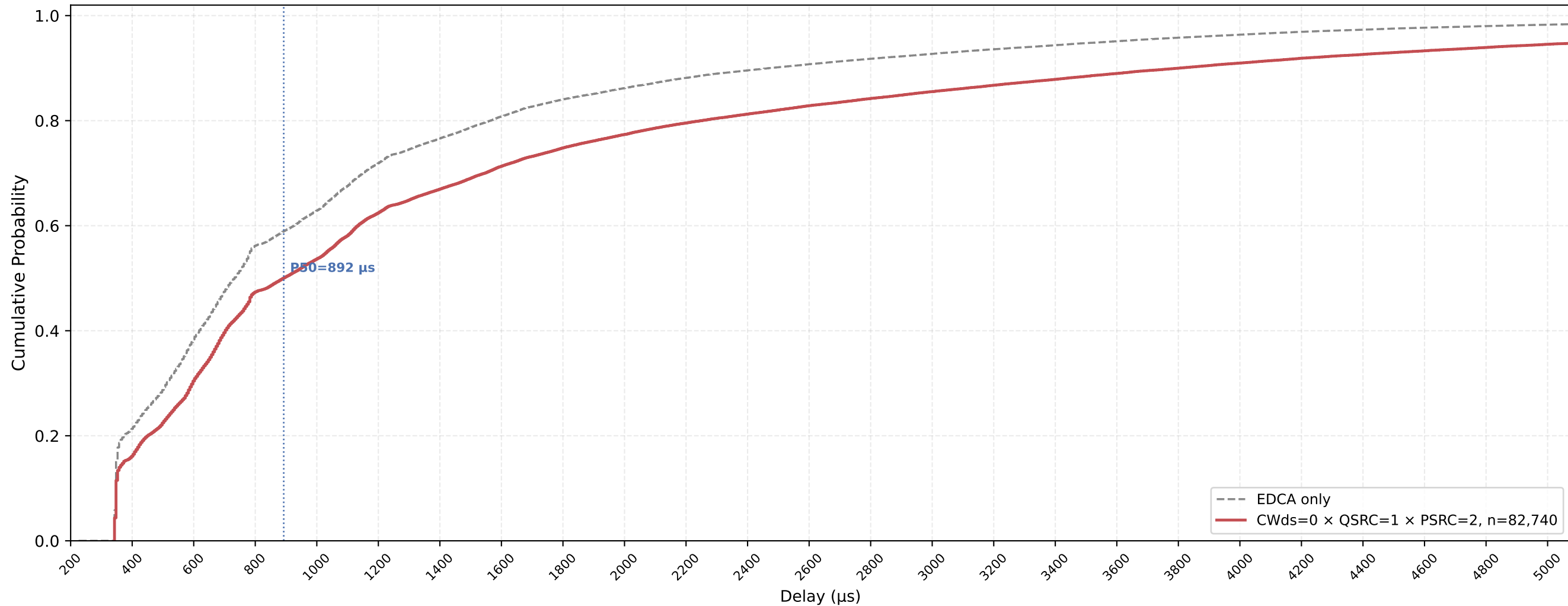
Legacy STA VO Delay CDF — CWds=0 × QSRC=1 × PSRC=2 nSta=30, nPedca=15, 0.5Mbps, avg of 10 runs
