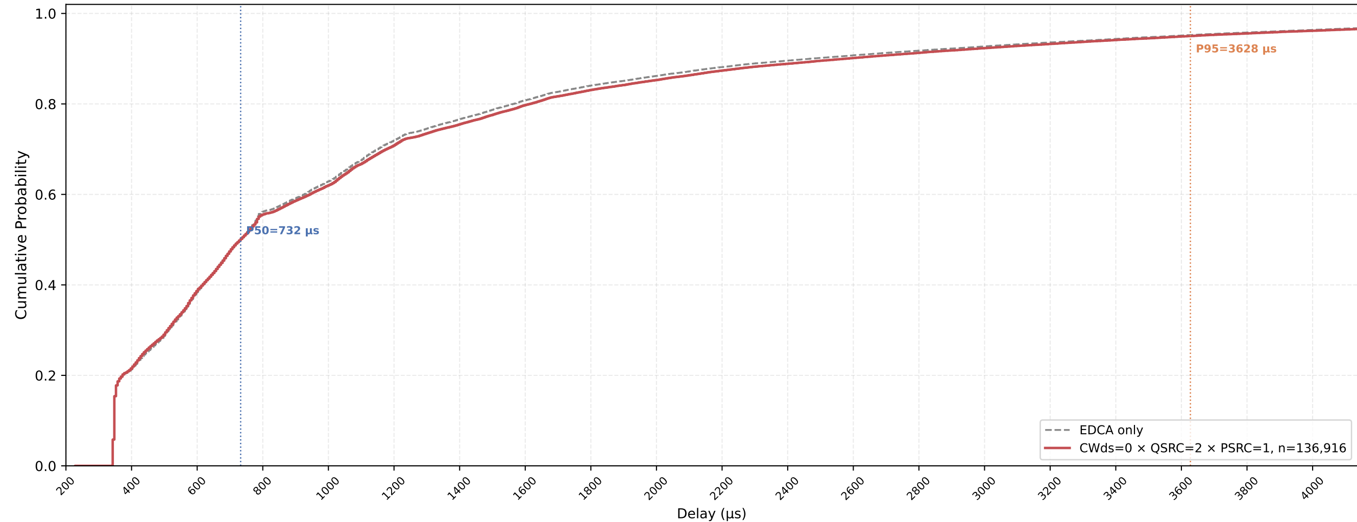
Legacy STA VO Delay CDF — CWds=0 × QSRC=2 × PSRC=1 nSta=30, nPedca=5, 0.5Mbps, avg of 10 runs
