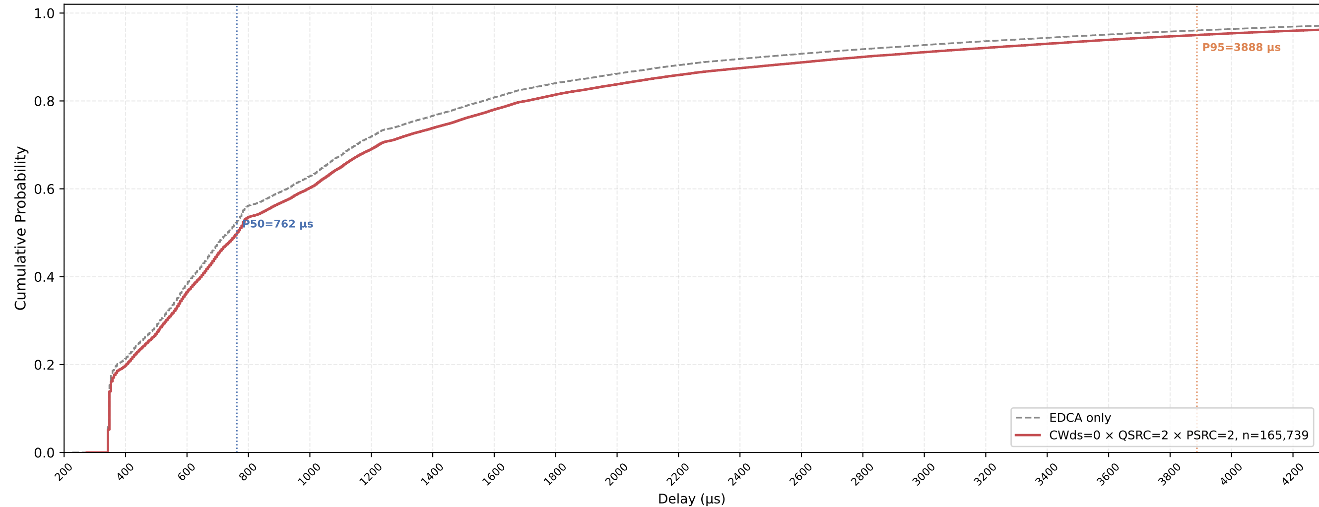
VO (all STAs) Delay CDF — CWds=0 × QSRC=2 × PSRC=2 nSta=30, nPedca=15, 0.5Mbps, avg of 10 runs
