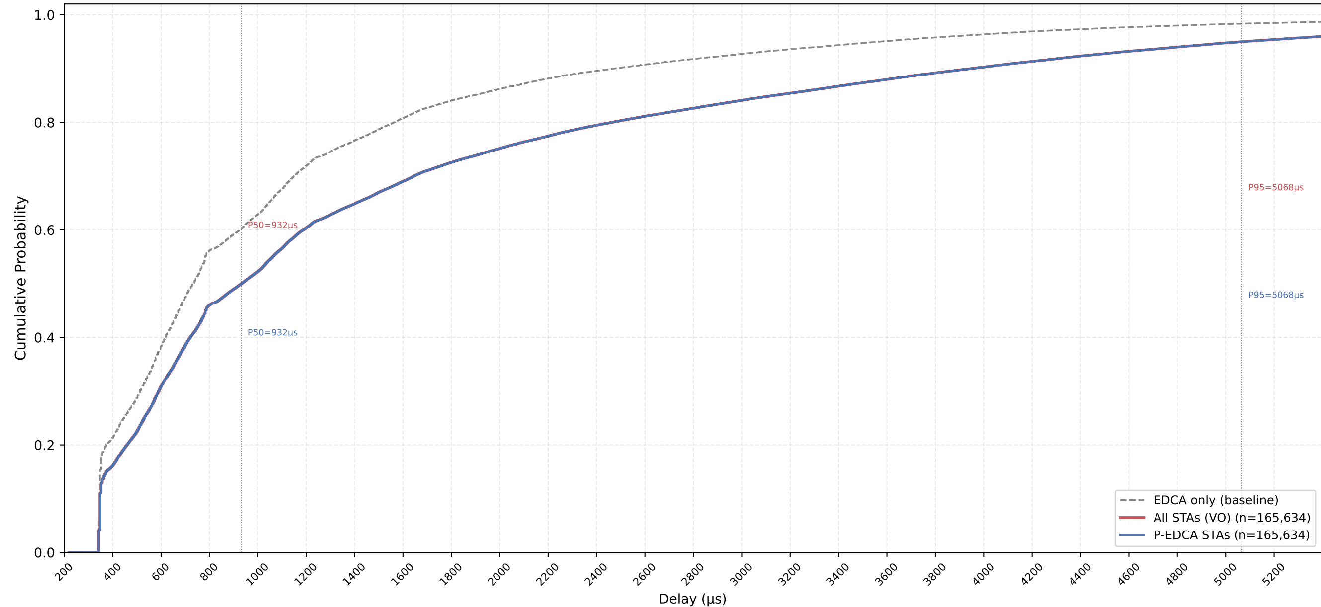
VO Delay CDF — P-EDCA / Legacy / All | CWds=0 × QSRC=2 × PSRC=3 nSta=30, nPedca=30/30, 0.5Mbps, avg of 10 runs
