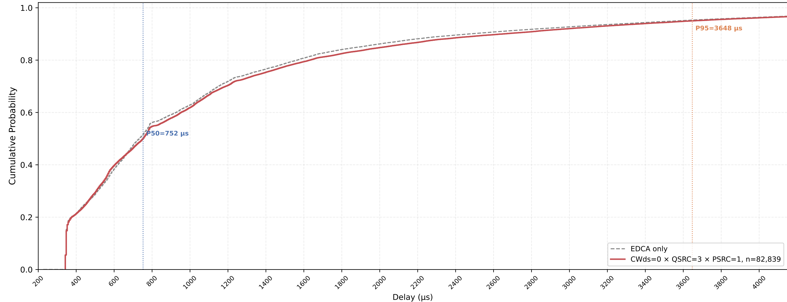
P-EDCA STA VO Delay CDF — CWds=0 × QSRC=3 × PSRC=1 nSta=30, nPedca=15, 0.5Mbps, avg of 10 runs
