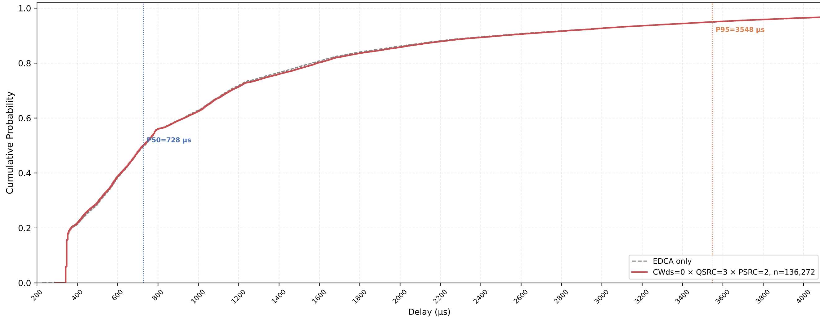
Legacy STA VO Delay CDF — CWds=0 × QSRC=3 × PSRC=2 nSta=30, nPedca=5, 0.5Mbps, avg of 10 runs
