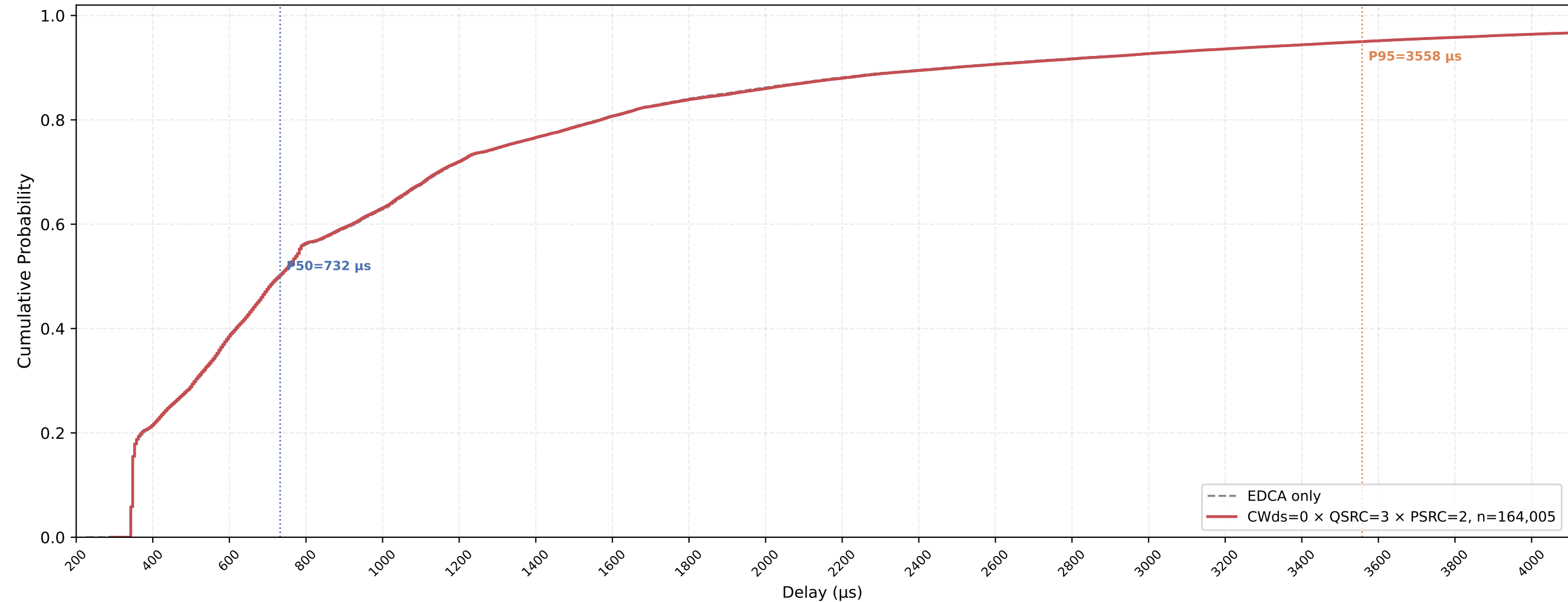
VO (all STAs) Delay CDF — CWds=0 × QSRC=3 × PSRC=2 nSta=30, nPedca=5, 0.5Mbps, avg of 10 runs
