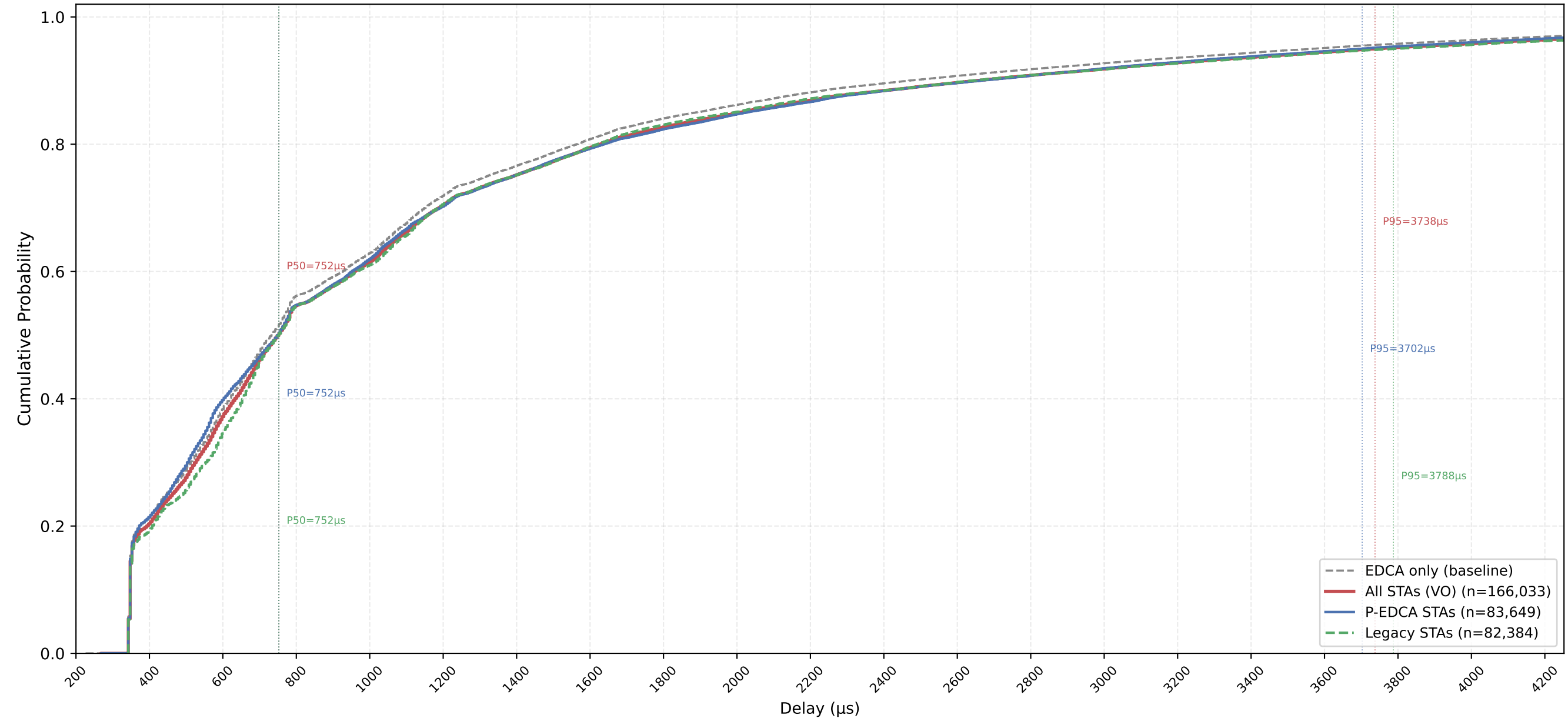
VO Delay CDF — P-EDCA / Legacy / All | CWds=0 × QSRC=3 × PSRC=3 nSta=30, nPedca=15/30, 0.5Mbps, avg of 10 runs
