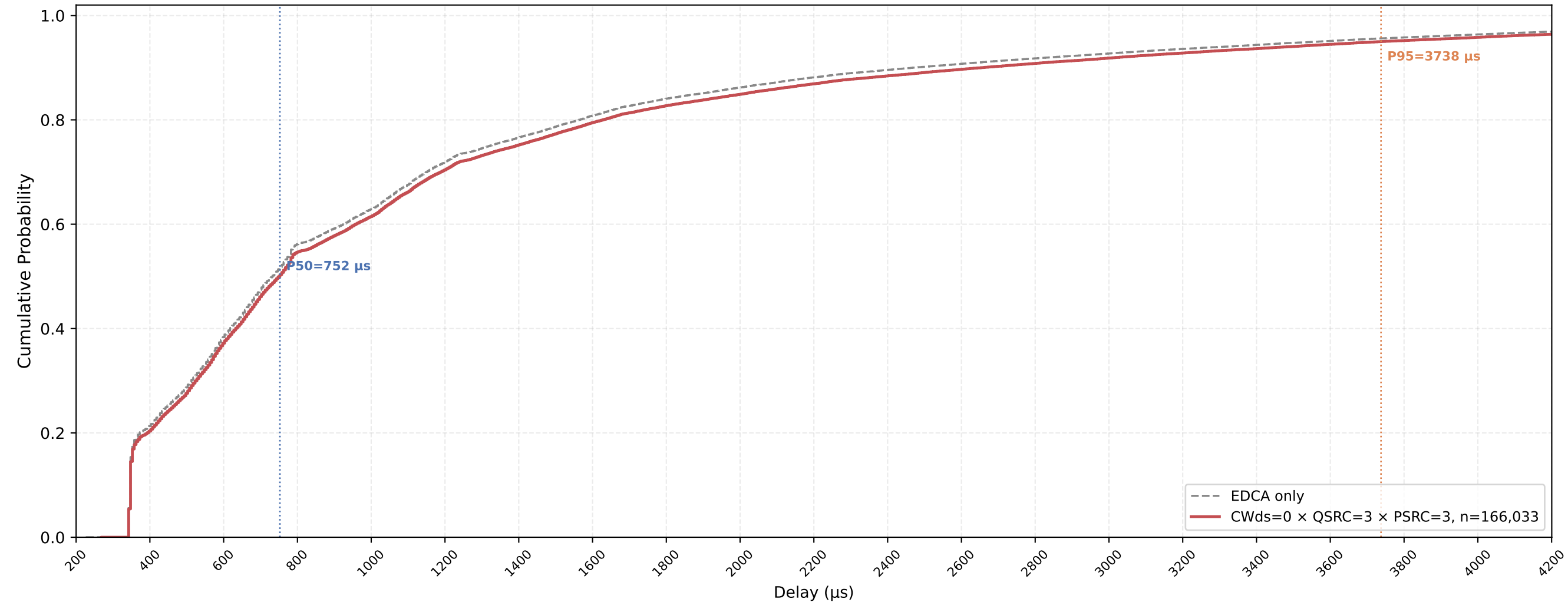
VO (all STAs) Delay CDF — CWds=0 × QSRC=3 × PSRC=3 nSta=30, nPedca=15, 0.5Mbps, avg of 10 runs
